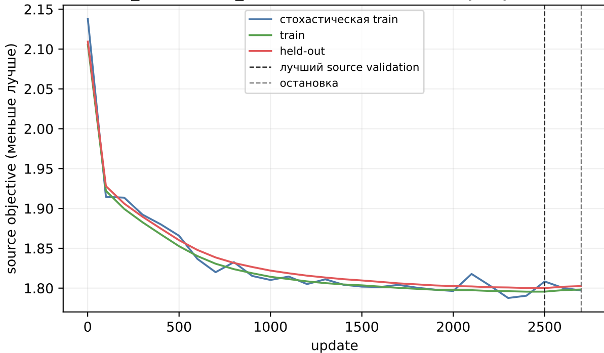
set_transformer_flow, seed 4103: source-only обучение
