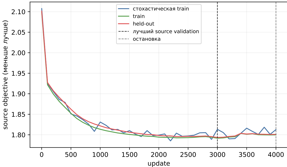
set_transformer_flow, seed 4105: source-only обучение
