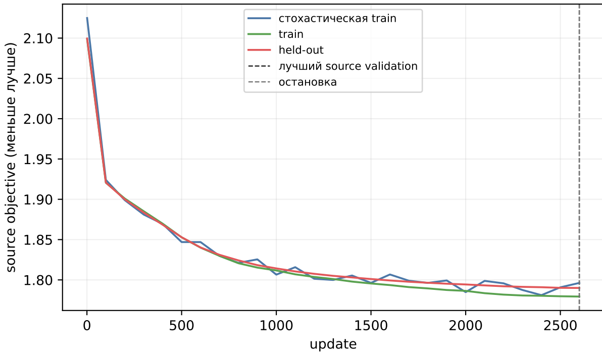
set_transformer_flow, seed 4107: source-only обучение
