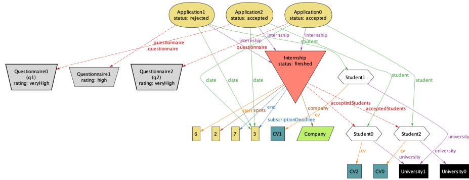
State 3
