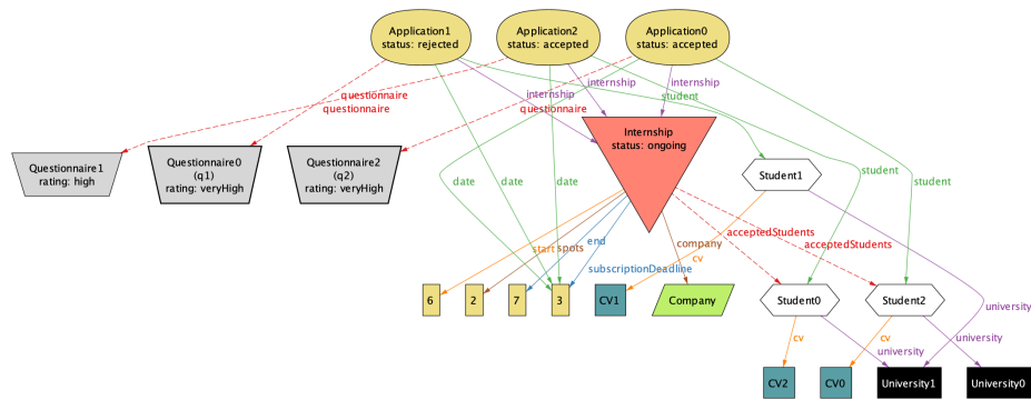
State 2
