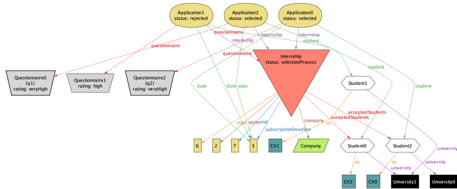
State 1
