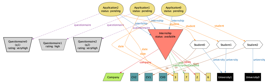
State 0
