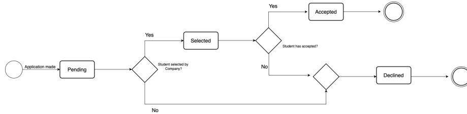
Application State Diagram
