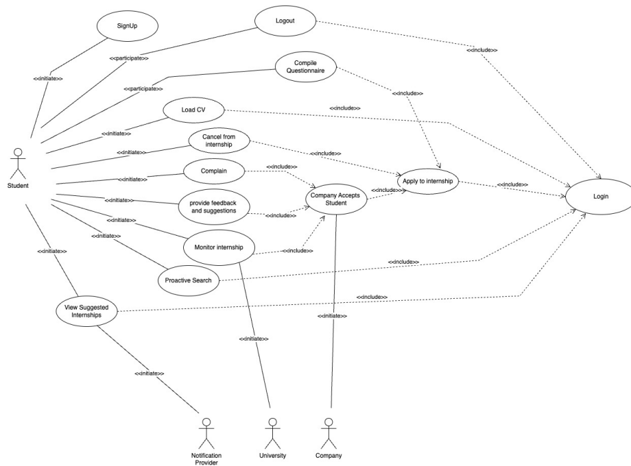
Student Use Case Diagram
