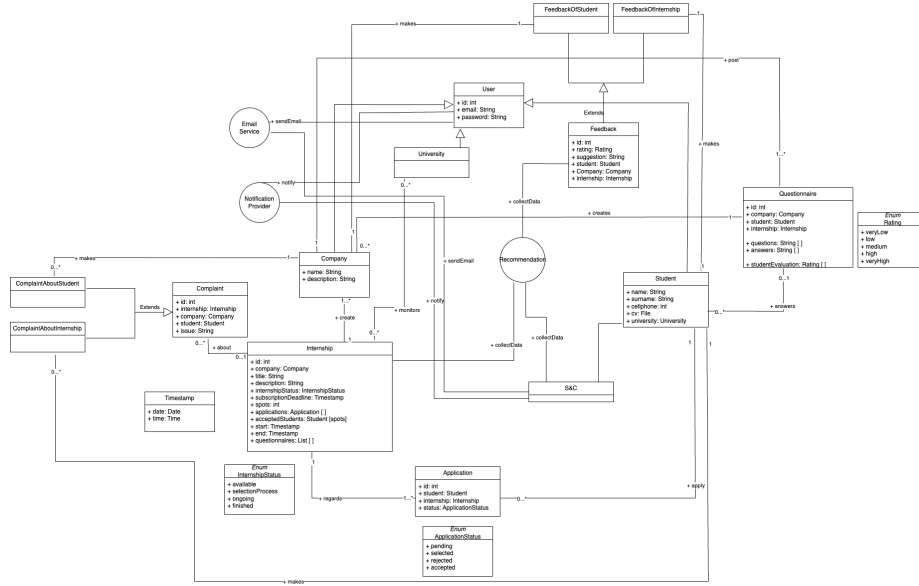
Domain Class Diagram
