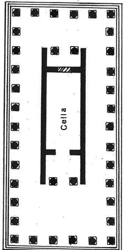
Pseudodipteros
