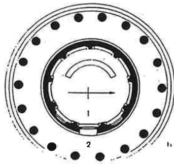
Olympia: Philippeion 1s. Typ. IX1
