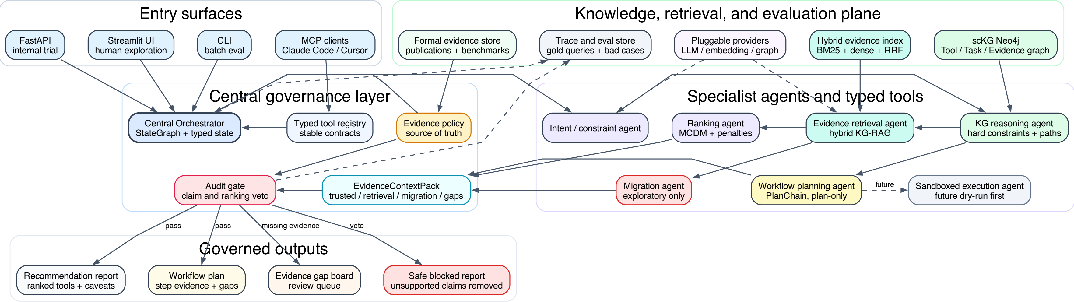
Figure 2. Target architecture: governed hybrid scientific agent
