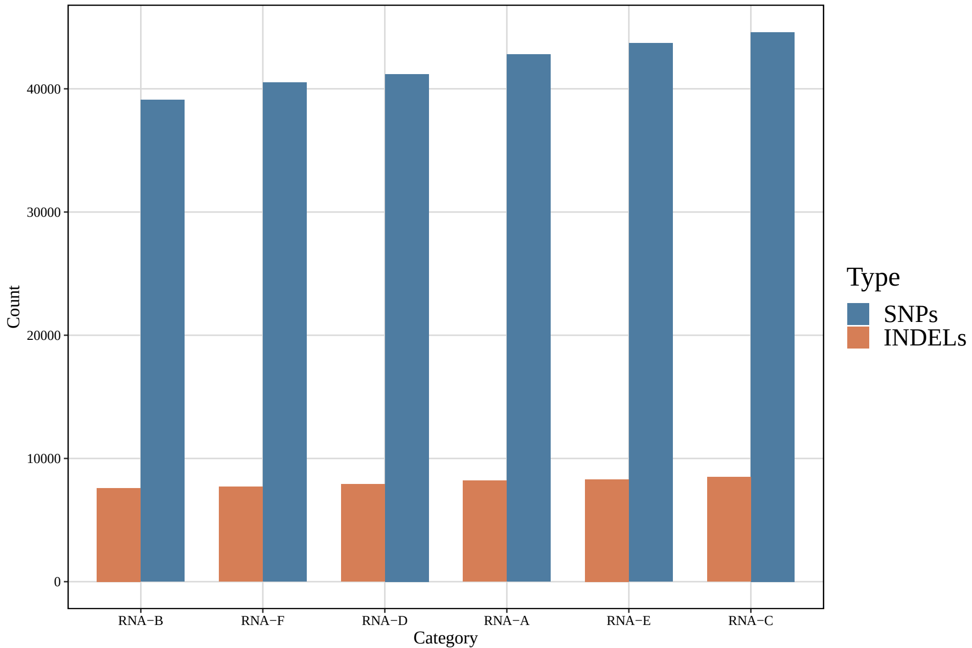
Variant counts
