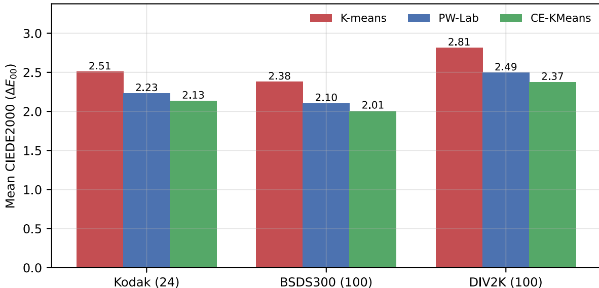
CIEDE2000 comparison across three datasets (K = 64)
