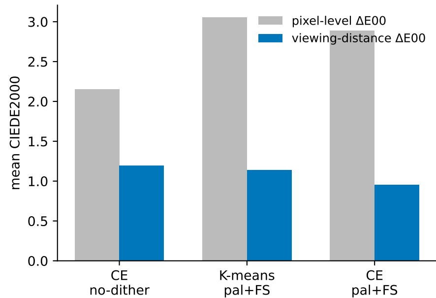
Kodak 24, K=64
