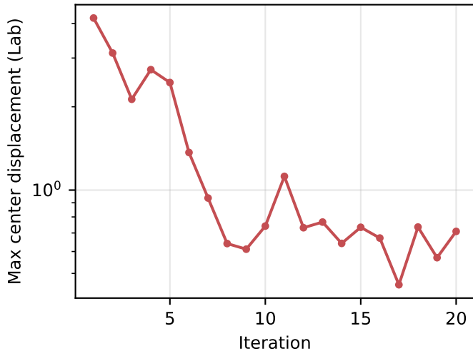
(b) Center movement
