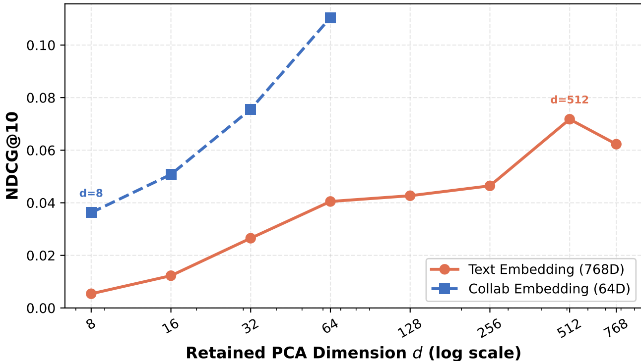
Figure 1: Information Density via PCA Truncation
