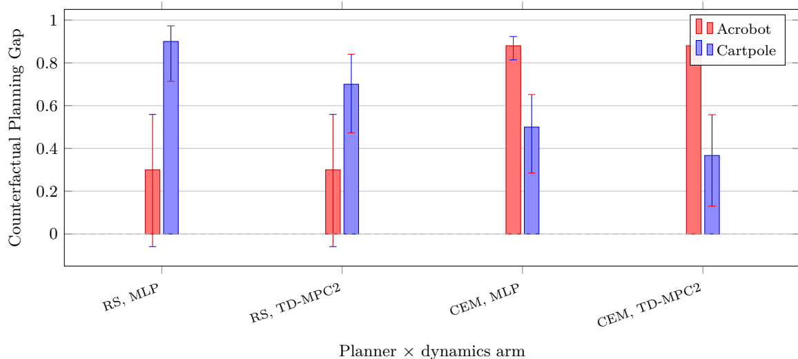
Figure 3: Cross-environment CPG with Agresti–Caffo 95% CI error bars. Same four planner-dynamics combinations on two envs. Sample sizes: Acrobot random-shooting cells at n = 10 , Acrobot CEM cells pooled at n = 150 , Cartpole all four cells pooled at n = 30 (TD-MPC2 model_size = 5). The MODEL BOTTLENECK verdict reproduces in every cell; the gap magnitude differs and ranks the four arm configurations consistently within each env. The TD-MPC2 arm on Cartpole reaches non-zero learned-arm success (0.200 random-shooting, 0.133 CEM), so the gap shrinks but stays bounded above zero – the metric tracks gap magnitude, not just gap presence.
