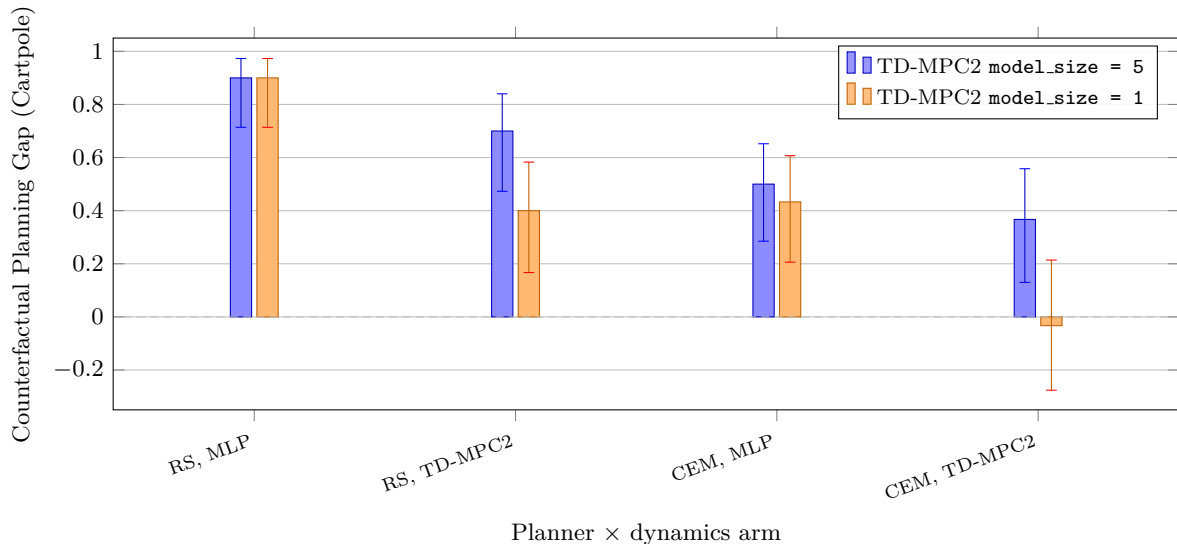
Figure 4: Cartpole capacity sweep at fixed 1 \times 10^6 -step training budget. Same four planner-dynamics combinations as Figure 3, comparing TD-MPC2 model_size = 5 (blue) against model_size = 1 (orange), n = 30 pooled per bar with asymmetric AC error bars. The CEM × TD-MPC2 cell at model_size = 1 (rightmost orange bar) is the only cell where the CI crosses zero: raw CPG = -0.033 , AC CI = [-0.28, +0.21] , verdict INCONCLUSIVE. Smaller-capacity TD-MPC2 closes the gap on Cartpole’s CEM oracle that the larger-capacity model does not – the metric reports this honestly rather than committing to a verdict the data does not support.
