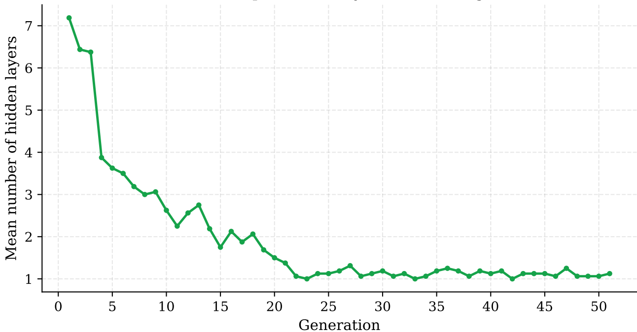
Architecture collapse: mean layer count over generations
