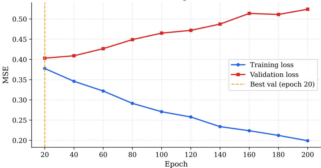
Baseline CNN: training vs validation loss
