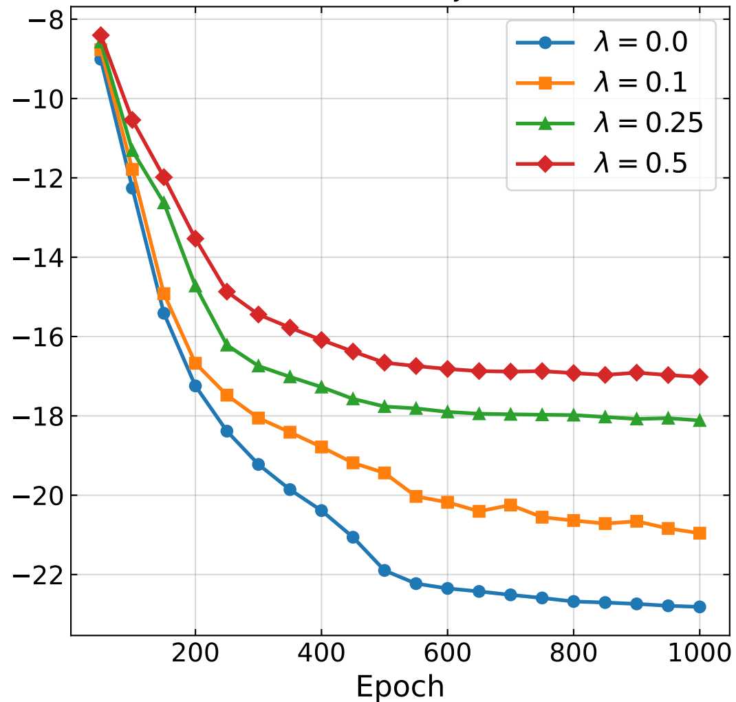
Evaluation Objective
