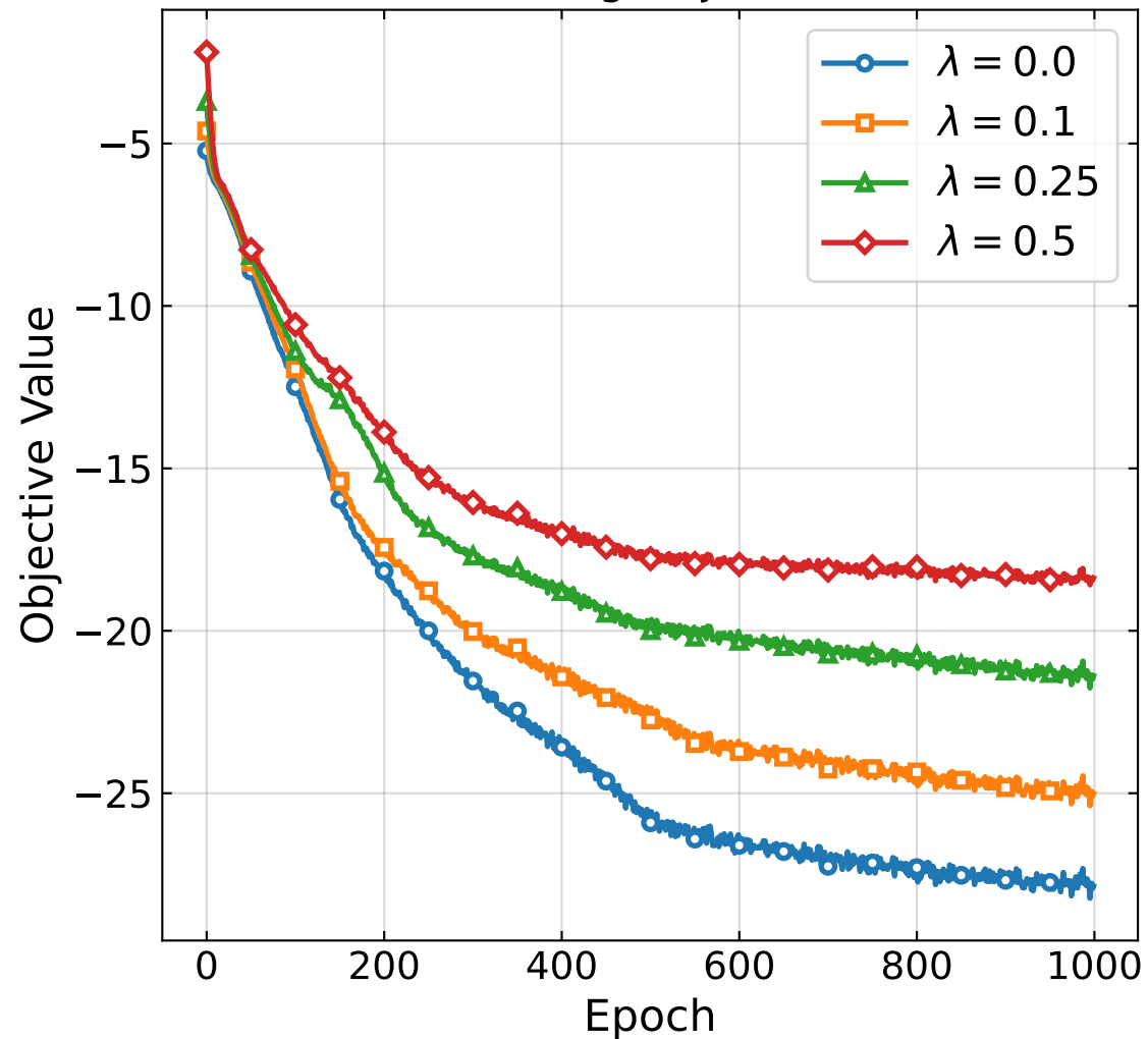
Training Objective
