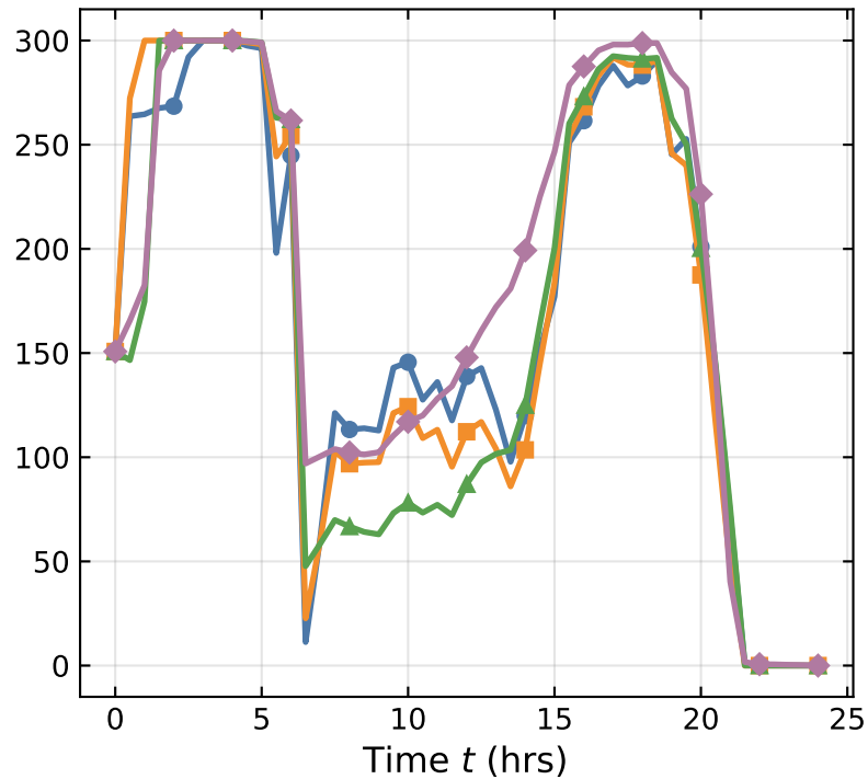
Stored energy \bar{E}_t
