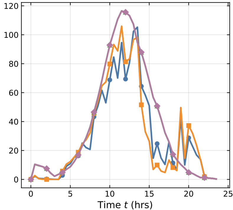
EV power allocation \bar{q}_t
