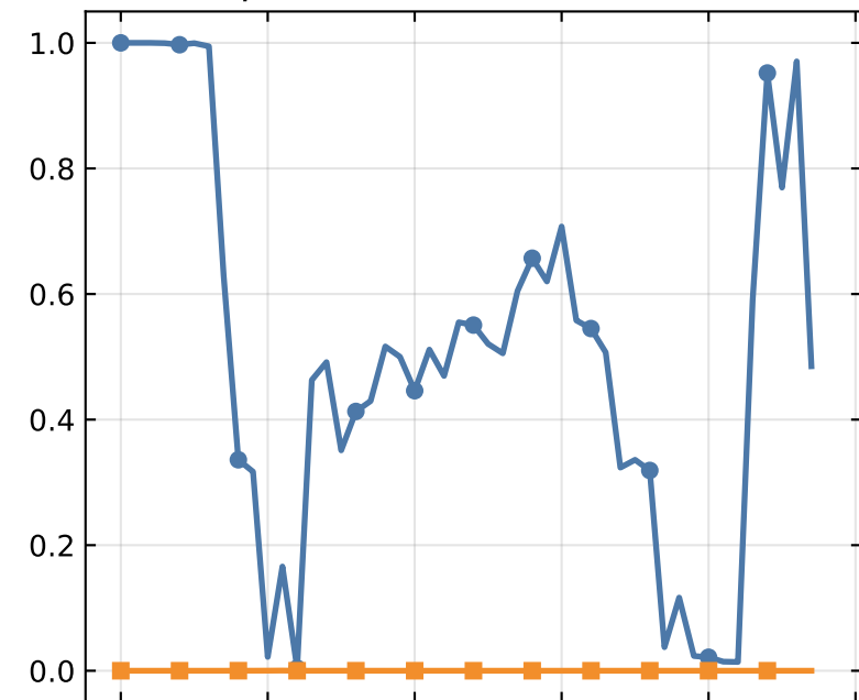
Purchased energy \bar{U}_t^b
