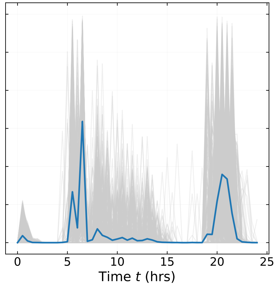
Trained
