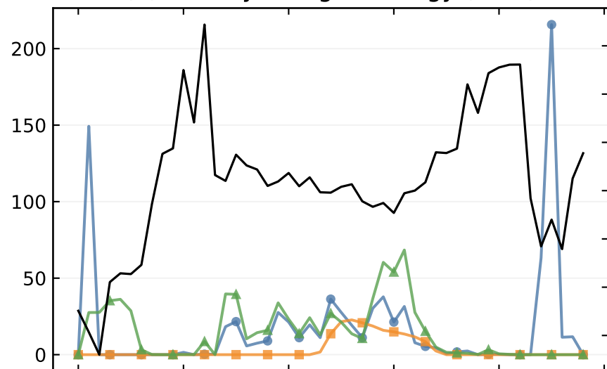
(c) Stored battery energy (kWh)
