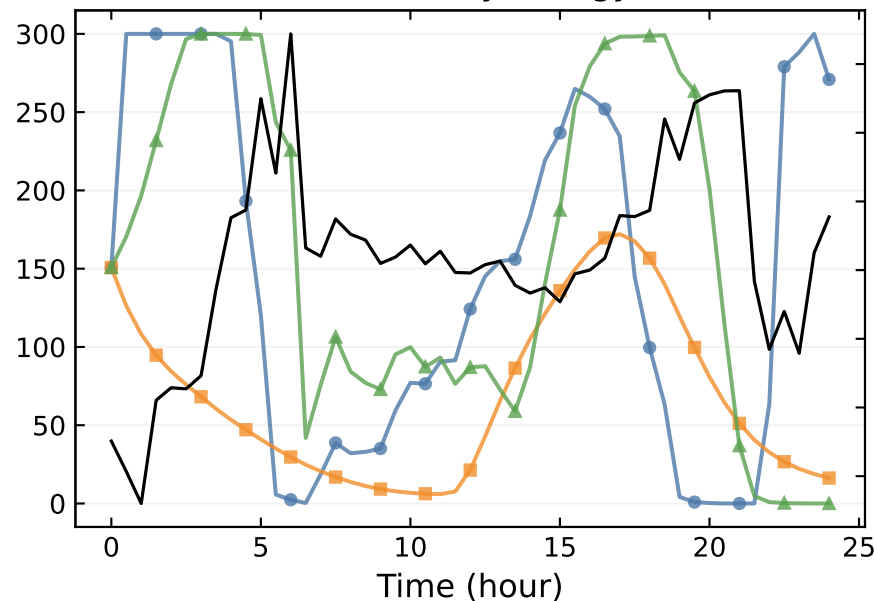
(c) Stored battery energy (kWh)
