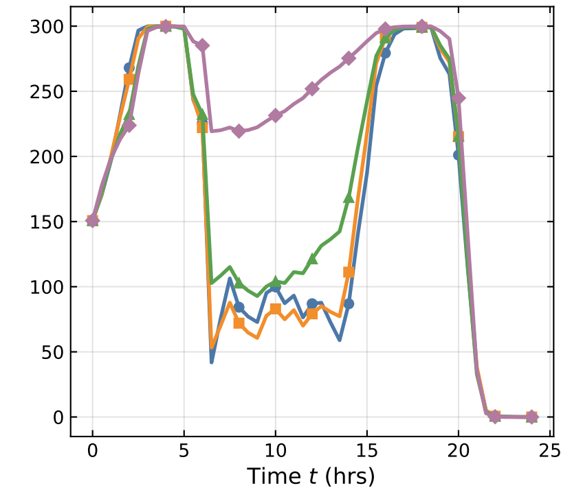
Stored energy \bar{E}_t
