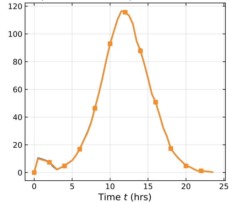
EV power allocation \bar{q}_t
