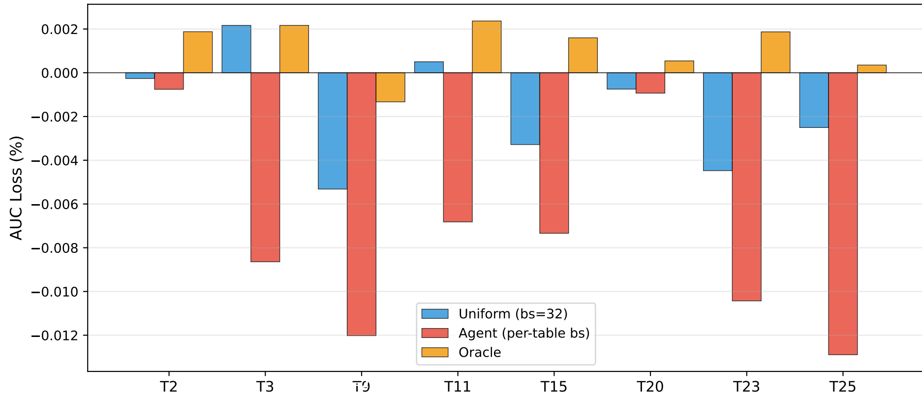
Per-Table Block Size: Agent vs Uniform vs Oracle (hf=1%, PCA sort, 4-bit DC)
