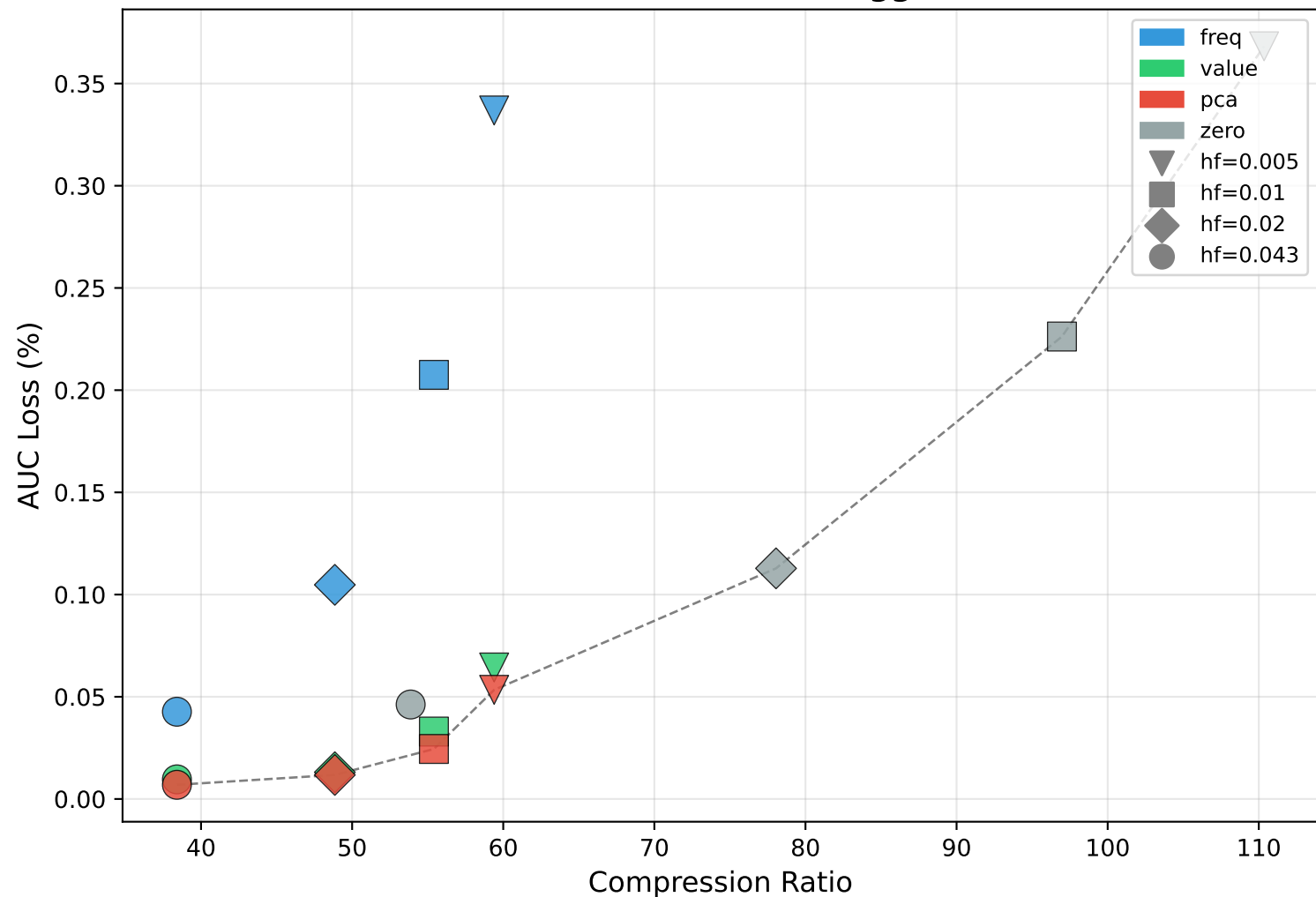
Compression Pareto Frontier by Sort Method (Actual AUC, Criteo Kaggle)
