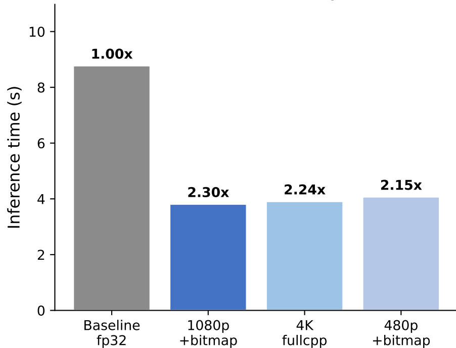
Inference Latency
