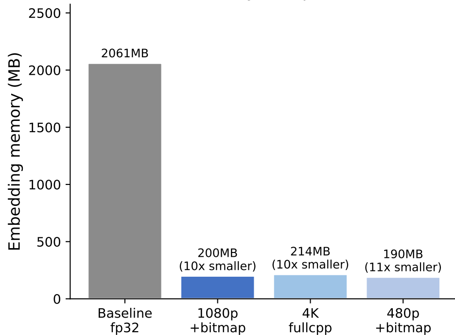
Memory Footprint
