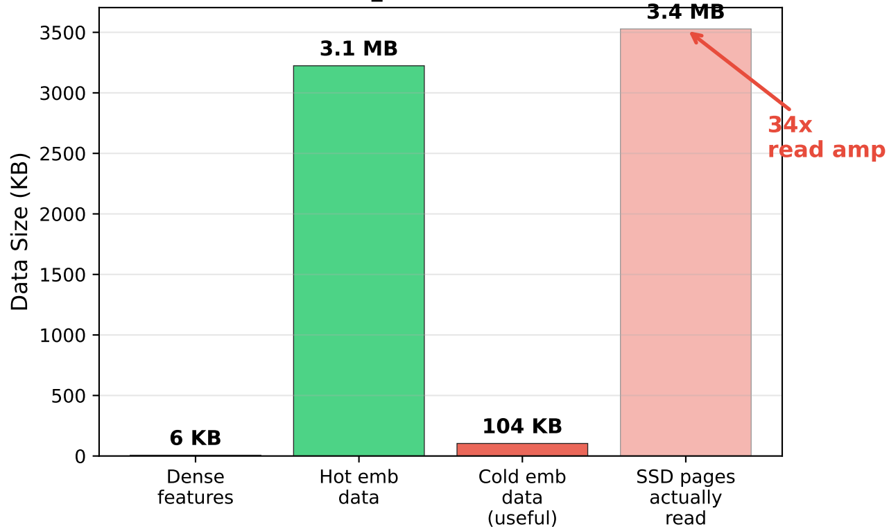
Data Accessed per Batch (batch_size=128, D=16)
