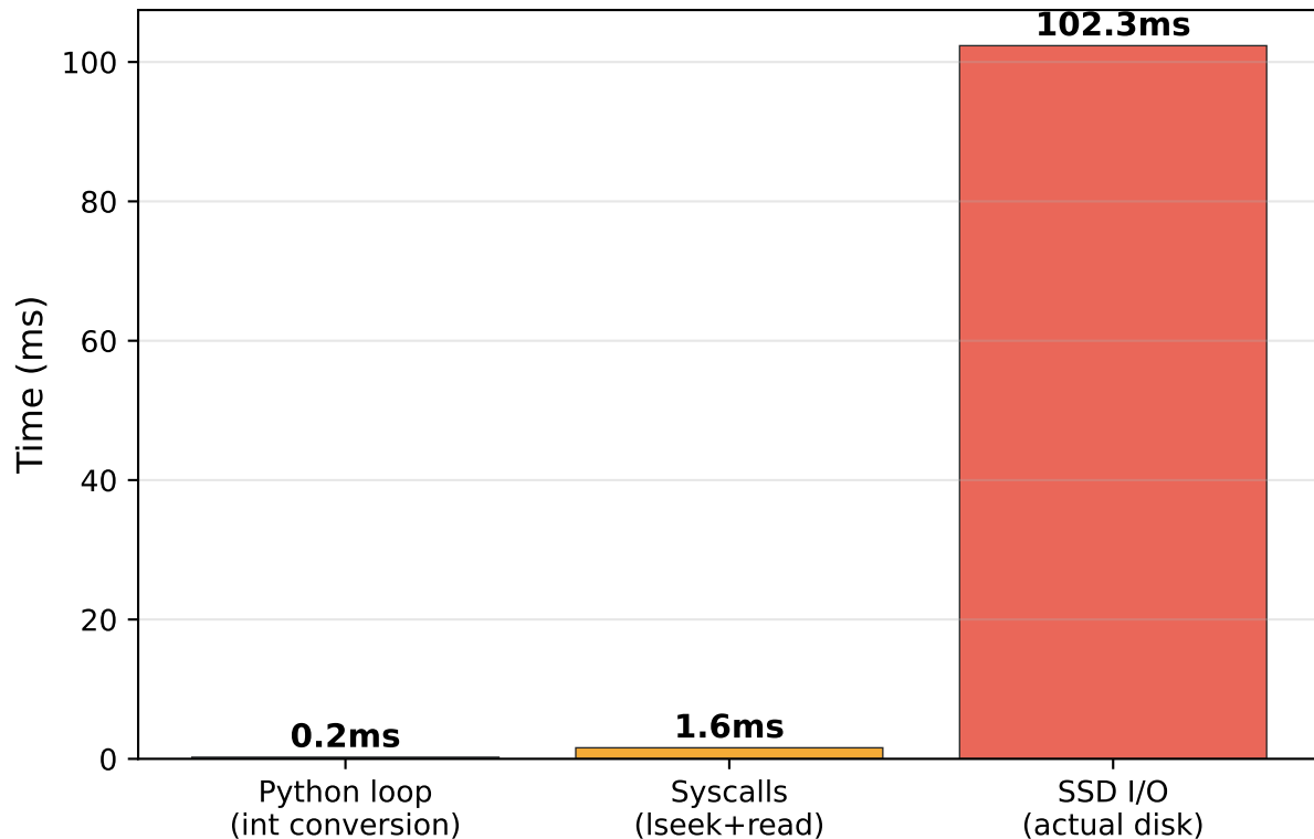
Overhead Breakdown (1,660 cold reads per batch)
