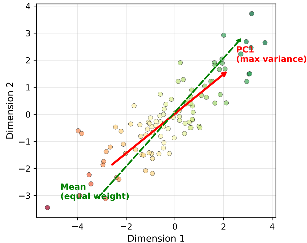
PCA vs Value Sort Direction (PCA finds max-variance axis)
