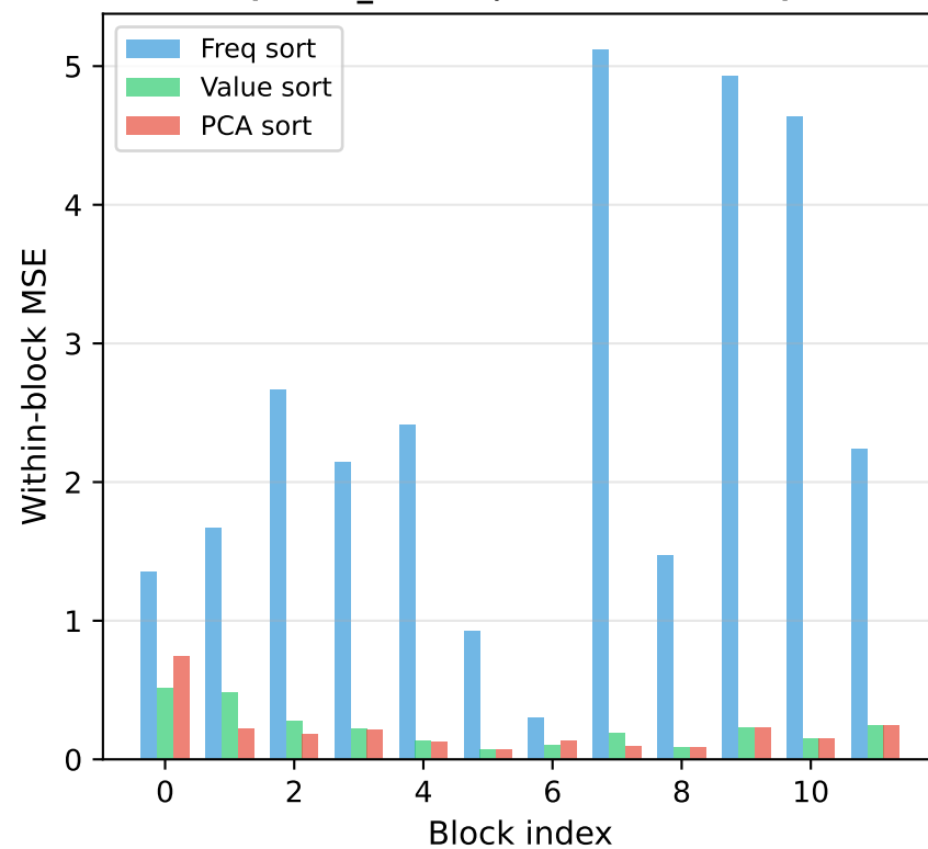
Block-Mean Approximation Error (block_size=8, lower = better)
