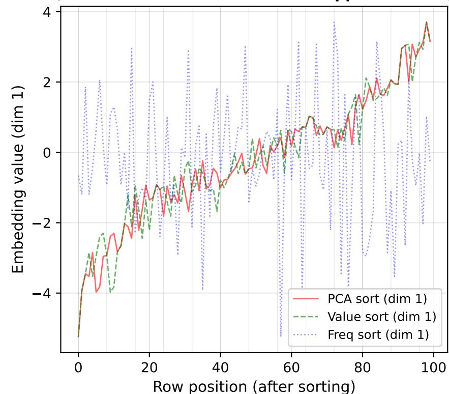
Sorted Embeddings: Smoothness Matters (smoother = better block-mean approximation)
