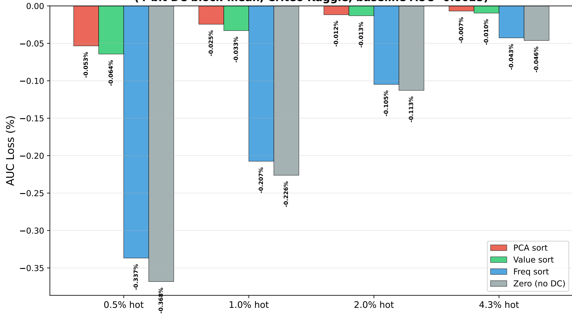
Sort Method Comparison: Real AUC Impact (4-bit DC block-mean, Criteo Kaggle, baseline AUC=0.8025)
