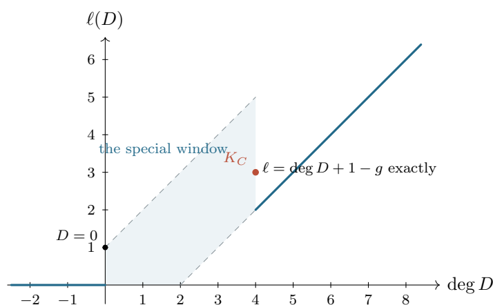
FIGURE 2. What \ell(D) can be, drawn for g = 3 . Left of degree 0: nothing. Right of degree 2g - 2 : the exact formula, no mystery. In the window between, \ell(D) ranges between the two dashed bounds ( \max(0, \deg D + 1 - g) from Riemann–Roch and \deg D + 1 from Proposition 7.5); the canonical class sits at the right edge with \ell(K_C) = g , one above the generic value.
