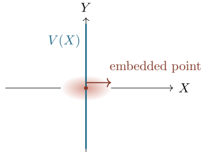
FIGURE 6. The affine k -variety defined by (X^2, XY) : the Y -axis with an embedded point at the origin. Away from the origin, a function in the ideal only has to vanish on the line. At the origin it must in addition vanish to second order in the X -direction (the arrow): its restriction to the X -axis is divisible by X^2 . This is the condition recorded by the embedded component (X^2, Y) , or equally by (X^2, XY, Y^2) .
