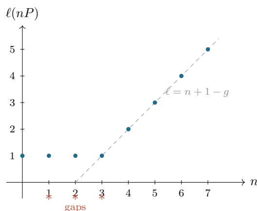
FIGURE 3. The Weierstrass staircase at a generic point of a genus-3 curve in characteristic 0: \ell(nP) stays flat exactly g = 3 times (at n = 1, 2, 3 , the gaps) and then climbs by 1 forever, joining the Riemann–Roch line. At special points – the Weierstrass points – the gap sequence is different, and it is a genuine fingerprint of the pair (C, P) . In positive characteristic even the generic gap sequence can differ from this picture; the gap theorem itself holds in every characteristic.
