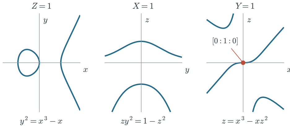
FIGURE 3. Three affine charts of the same smooth cubic. The point [0 : 1 : 0] , absent from the left-hand chart, is the marked origin in the right-hand chart. Each drawing is a bounded window in its affine plane.
