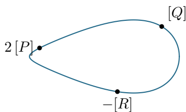
FIGURE 1. A divisor made visible: D = 2[P] + [Q] - [R] , of degree 2. A global section of \mathcal{O}(D) is a rational function that is allowed a double pole at P and a simple pole at Q , and is required to vanish at R . Riemann–Roch (Theorem 7.14) is the exact count of such functions.
