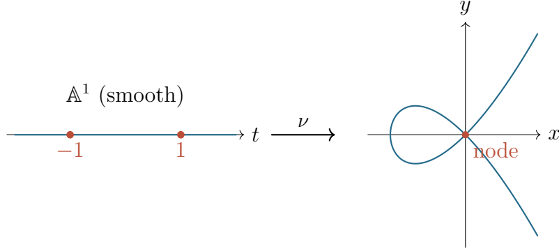
FIGURE 7. The normalization \nu: t \mapsto (t^2 - 1, t(t^2 - 1)) of the nodal cubic y^2 = x^2(x + 1) : enlarging the coordinate ring k[t^2 - 1, t(t^2 - 1)] to its integral closure k[t] separates the two branches, pressing the two smooth points t = \pm 1 onto the node.
