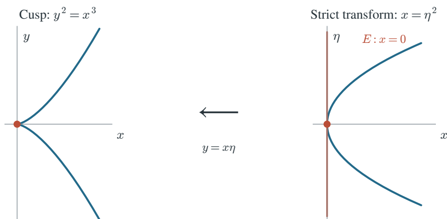
FIGURE 1. One blow-up of the cusp. In the chart y = x\eta , the strict transform is the smooth parabola x = \eta^2 . The exceptional divisor E = V(x) is red. Smoothness has been achieved, but the strict transform is still tangent to E ; these are two different geometric questions.
