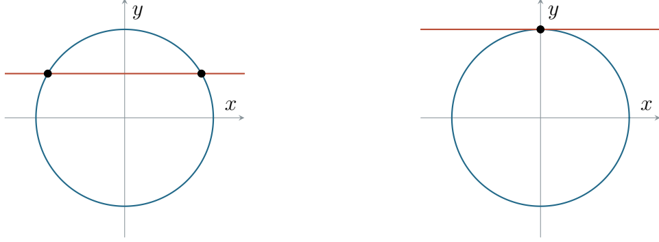
FIGURE 4. Intersections of a line with the circle x^2 + y^2 = 1 in \mathbb{A}^2 .
