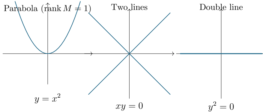
FIGURE 2. A parabola, a pair of lines, and a double line. The last two equations are degenerate conics.
