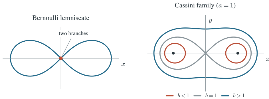
FIGURE 4. Two classical quartics. The Bernoulli lemniscate is rationally parametrized, even though it is not a conic. Cassini ovals are included for a different reason: they show how the real shape of a plane curve can change inside one algebraic family.
