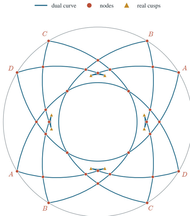
FIGURE 7. The real dual curve of the Trott quartic, drawn in a compact projective-disk model of the dual plane. The red points are all 28 nodes of C^\vee , corresponding to the 28 real bitangent lines of the original quartic. The orange triangles mark the images of the 8 real inflection points highlighted in Figure 6; these become real cusps of the dual curve. The remaining flexes are non-real in this example. Antipodal boundary points are identified: each of the four boundary nodes is drawn twice, with matching labels A, B, C, D . Thus the 32 red marks represent 28 projective points.
