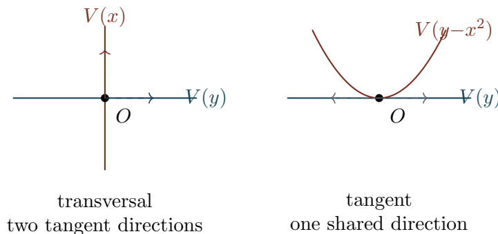
FIGURE 1. The same set-theoretic picture — one intersection point at the origin — but two different local geometries. Left: V(y) and V(x) cross transversally; their tangent directions are independent. Right: V(y) is tangent to the parabola V(y - x^2) ; both share the horizontal tangent direction. The local ring records the difference: dimension 1 in the first case, dimension 2 in the second.
