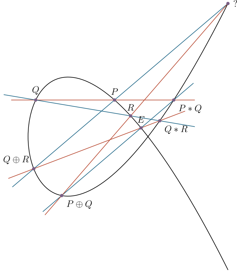
FIGURE 5. The associativity construction. The rows and columns of the 3 \times 3 square are lines; both ways of computing the sum end at the point marked ?.
