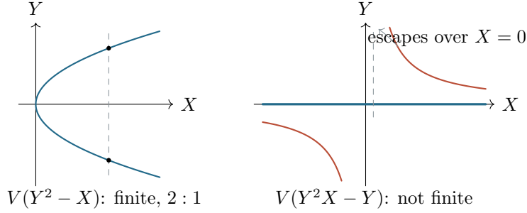
FIGURE 4. Finite versus not finite. Left: the parabola projects onto the X -axis with all fibres of the same size, counted properly; Y is monic over k[X] . Right: the union of the hyperbola and the X -axis also projects with finite fibres, but one branch runs away to infinity over X = 0 , and Y satisfies no monic equation. Noether normalization says a linear change of coordinates always repairs this.
