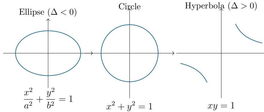
FIGURE 1. Non-degenerate affine conics.
