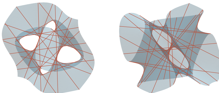
Clebsch cubic: line overlay
