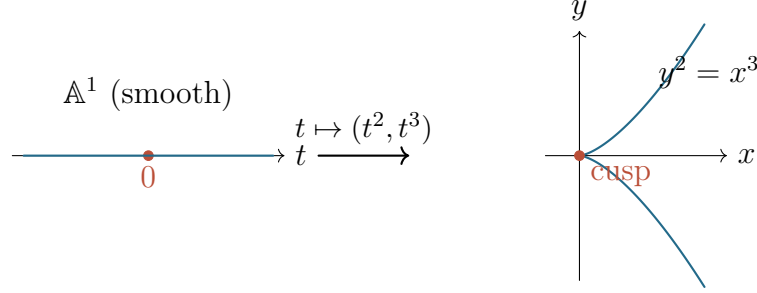
FIGURE 5. The parametrization t \mapsto (t^2, t^3) maps the smooth line \mathbb{A}^1 bijectively onto the cuspidal cubic y^2 = x^3 . The smooth origin of \mathbb{A}^1 maps to the cusp at (0,0) : parametrizations can cover singular points without reflecting their local geometry.
