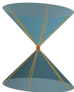
\mathbb{F}_2 : contraction to a cone
