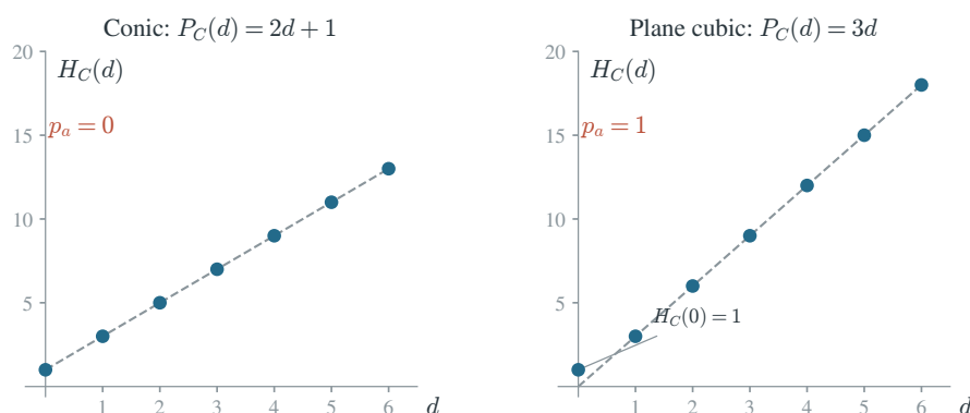
FIGURE 2. The Hilbert functions of a plane conic and a plane cubic (dots), with their Hilbert polynomials (dashed lines). The slope gives the degree; the constant term is 1 - p_a . For the cubic, H_C(0) = 1 but P_C(0) = 0 : agreement with the polynomial is only required in sufficiently large degrees.
