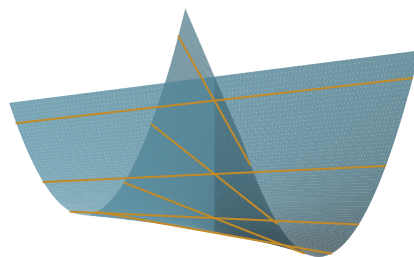
Cubic scroll: a projection
