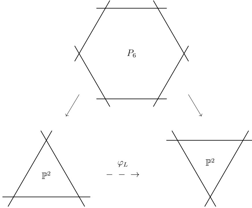
FIGURE 5. The plane Cremona map factors through the blow-up of its three base points.
