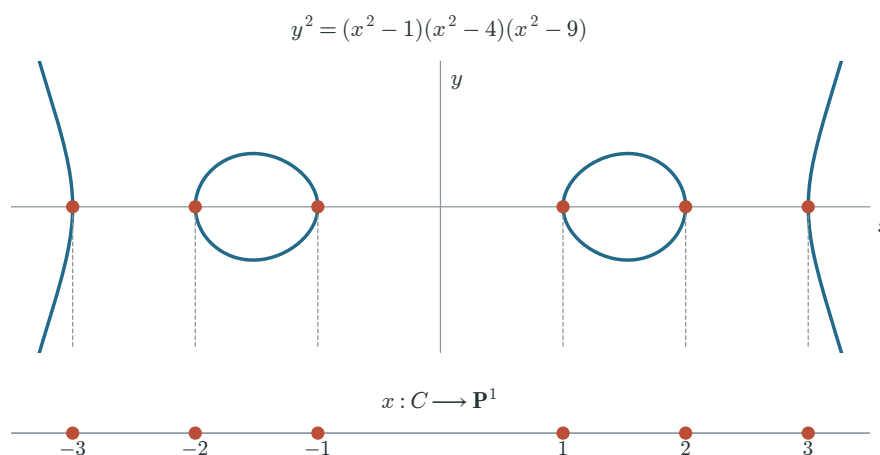
FIGURE 4. Six real branch values of a degree-two map to \mathbb{P}^1 . The upper picture shows only the real affine points of the genus-2 curve; the vertical scale is compressed. At each marked point the two real arcs join, and locally x - a is a unit times y^2 , so e = 2 . Intervals with no real points above them still have two complex points in each fibre, just as in the Noether-normalization picture of Chapter 2 (Figure 5).
