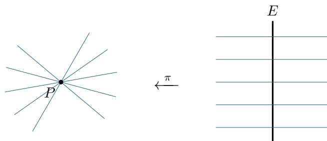
FIGURE 5. Blowing up the base point of the pencil. On \mathrm{Bl}_P \mathbb{P}^2 the strict transforms of the lines through P are disjoint – the computation (H - E)^2 = 0 made visible – and each meets the exceptional curve E once, in the point of E recording its direction at P . Together they are the fibres of the morphism \mathrm{Bl}_P \mathbb{P}^2 \rightarrow \mathbb{P}^1 .
