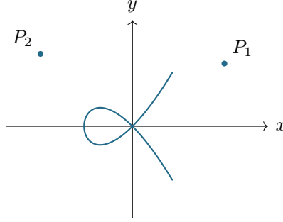
FIGURE 1. A typical Zariski-closed subset of \mathbb{A}^2 : a curve together with finitely many extra points. The complement of this thin set is a single huge open set, dense in the plane.
