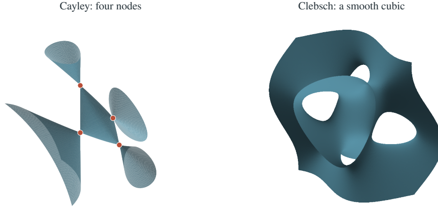
FIGURE 2. The singular Cayley cubic and the smooth Clebsch diagonal cubic. The four marked points on the Cayley model are its nodes; the Clebsch model has no singularities. These are bounded windows in real affine charts, so the surfaces continue beyond the edges. The 27 lines on the Clebsch surface are shown separately in Figure 6.
