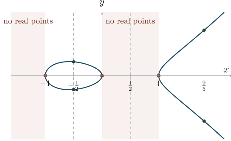
FIGURE 5. Noether normalization for the curve C: y^2 = x^3 - x , via the projection \pi: (x, y) \mapsto x . The real points lie over [-1, 0] \cup [1, \infty) . Green fibres (at x = -\frac{1}{2} and x = \frac{9}{5} ) have 2 real points; red points (at x = 0, \pm 1 ) are fibres with exactly 1 point, where the two sheets collide: these are the branch points of the cover. Over x < -1 and 0 < x < 1 (shaded; e.g. the grey fibre at x = \frac{1}{2} , where x^3 - x = -\frac{3}{8} ) there are no real points, though over an algebraically closed k every fibre is nonempty. Algebraically, k[C] = k[x, y]/(y^2 - x^3 + x) is finite over k[x] \cong k[\mathbb{A}^1] with integral generator y (satisfying y^2 = x^3 - x ), making \pi a finite surjection of degree 2.
