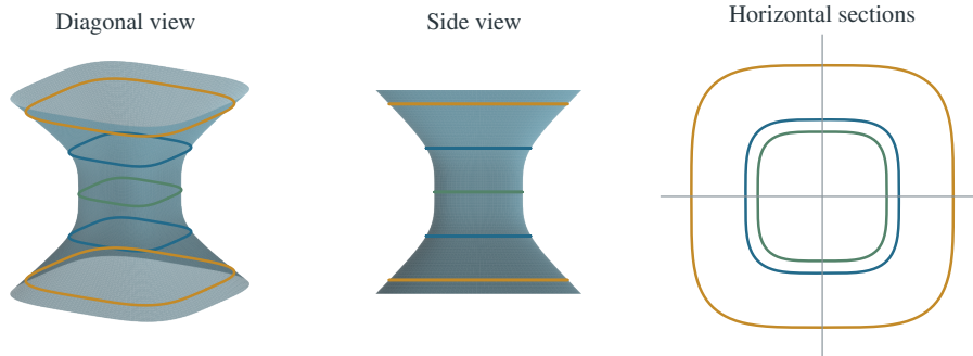
FIGURE 3. The diagonal quartic surface x^4 + y^4 - z^4 = 1 seen from three perspectives. Left : diagonal view with horizontal section curves at z = 0 (green waist, squircle x^4 + y^4 = 1 ), z = \pm 1 (blue), and z = \pm 2 (gold); the coloured curves are the cross-sections x^4 + y^4 = 1 + z^4 , which are squircles that grow as |z| increases. Centre : side view ( y -axis direction), showing the two arms funnelling outward from the waist as z \rightarrow \pm\infty . Right : top view (looking down the z -axis), showing the nested squircle cross-sections — all the same shape, just scaled by (1 + z^4)^{1/4} .
