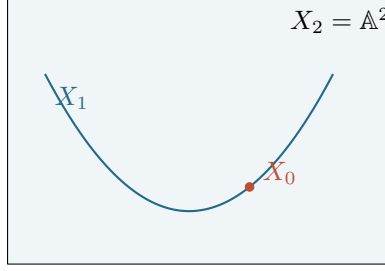
FIGURE 3. A chain of irreducible closed subsets witnessing \dim \mathbb{A}^2 \geq 2 : a point X_0 on a curve X_1 in the plane X_2 . That no longer chain exists – so that the dimension is exactly 2 – is the substance of the dimension theory developed in this section and Appendix C.
