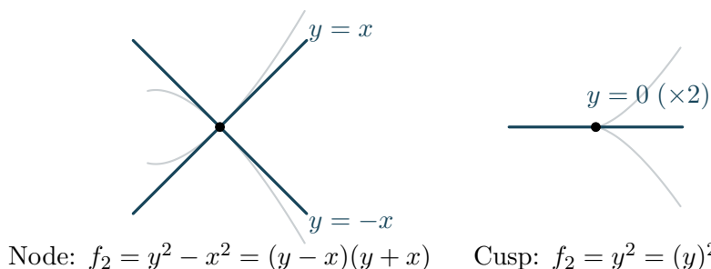
FIGURE 4. Tangent cones at the origin. The curve (grey) recedes into the background; the tangent cone (blue) is the leading-order shape. Left: the node's leading form y^2 - x^2 splits into two coprime linear factors, giving two tangent directions. Right: the cusp's leading form y^2 is a perfect square, giving one direction with multiplicity 2. The key contrast is coprimeness, not multiplicity.
