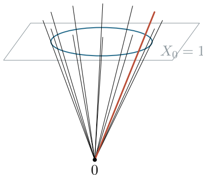
FIGURE 1. A homogeneous ideal cuts out a cone in \mathbb{A}^{n+1} : with every point it contains the whole line through that point and the origin (here, the cone in \mathbb{A}^3 over a conic). A projective point of V(I) is such a line (one drawn in red), and slicing with the plane X_0 = 1 recovers the affine picture; a line parallel to that plane would be invisible in the slice – a point at infinity.
