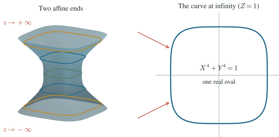
FIGURE 8. Harnack's theorem applied to the diagonal quartic x^4 + y^4 - z^4 = 1 ( d = 4 ). The two affine ends on the left approach the same oval of the curve at infinity, drawn on the right in the chart Z = 1 . Thus r_\infty = 1 , and the sharper bound using this particular boundary is \#\{\text{arms}\} \leq 2r_\infty = 2 , attained here. For an arbitrary smooth plane quartic at infinity, Harnack gives r_\infty \leq 4 .
