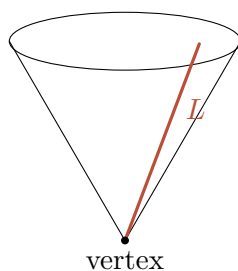
FIGURE 4. The quadric cone Q = V(xy - z^2) , the simplest singular surface. The ruling L = V(x, z) \subset Q is a prime Weil divisor that is not Cartier at the vertex: no single equation cuts it out there. Its double is: the function x vanishes on Q exactly along L , to order two, so \text{div}(x) = 2L . Proposition 8.2 says smoothness rules out exactly this behaviour.
