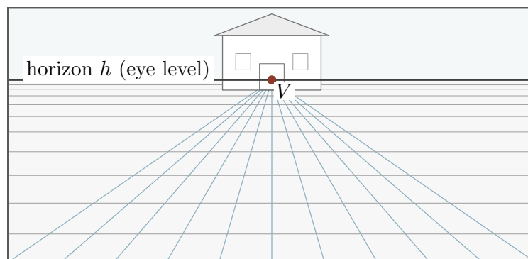
FIGURE 2. One-point perspective as a projective construction. The blue orthogonals, parallel on the ground, converge to their vanishing point V . The gray crosswise edges are parallel to the picture plane and remain parallel in the finite picture. The horizon h is the image of the ground plane's line at infinity.
