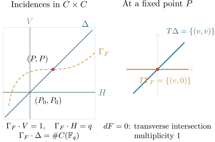
FIGURE 7. The curves used in the Weil-bound argument. Left: an incidence schematic, not a real plot or a topological model of C \times C . The fibre \Gamma_F \cap H has length q , although it has only one geometric point. Right: at any fixed point P , the two tangent lines are distinct because dF = 0 , so \Gamma_F \cdot \Delta counts that point once. The marked fixed point illustrates the local argument; its existence is not assumed.
