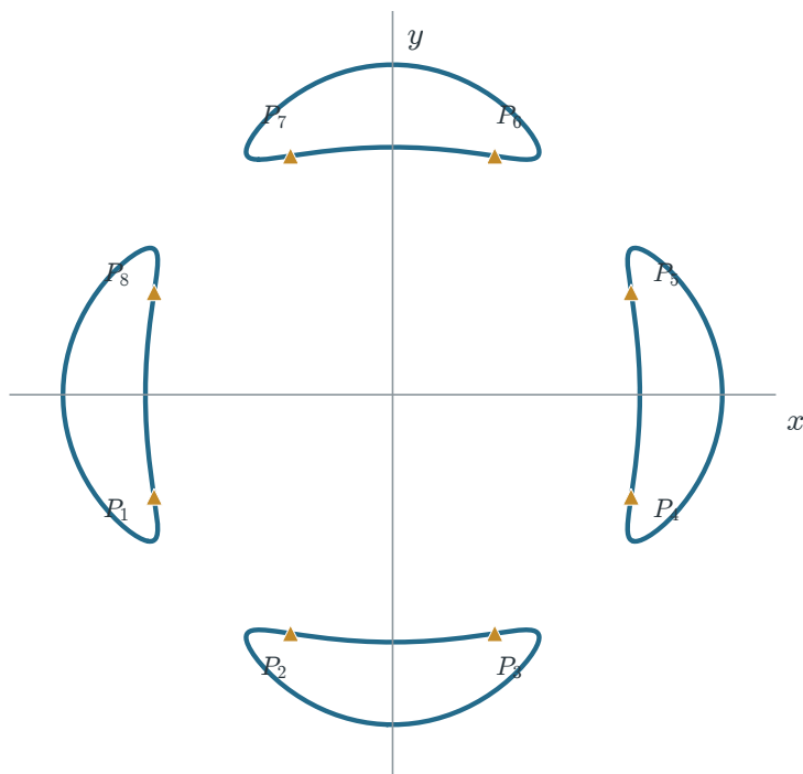
FIGURE 6. The real Trott quartic with its 8 real inflection points highlighted. A smooth quartic has 24 inflection points over an algebraically closed field, counted with multiplicity; for this real model the remaining flexes are non-real. These highlighted points will become the real cusps of the dual curve in Figure 7.
