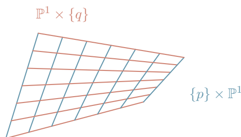
FIGURE 3. A patch of the Segre quadric \Sigma_{1,1} = V(Z_{00}Z_{11} - Z_{01}Z_{10}) \subset \mathbb{P}^3 , the image of \mathbb{P}^1 \times \mathbb{P}^1 . The two families of lines are the images of the vertical and horizontal copies of \mathbb{P}^1 : through every point passes exactly one line of each family, two lines of the same family are disjoint, and lines of different families meet in one point.
