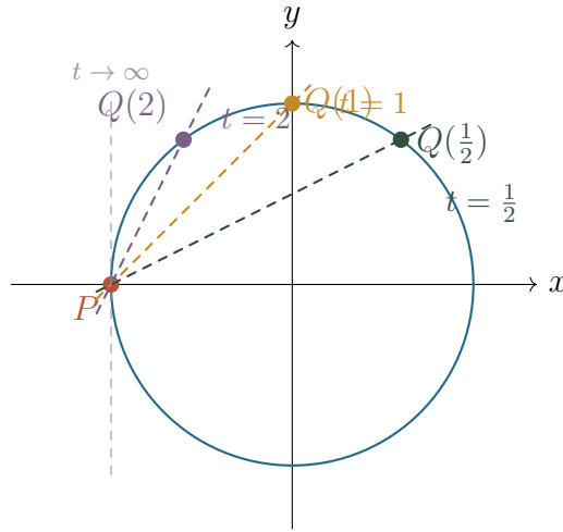
FIGURE 3. Parametrizing the unit circle by lines through P = (-1, 0) . A line through P with slope t has equation y = t(x + 1) ; its second intersection with x^2 + y^2 = 1 is the point Q(t) = (\frac{1-t^2}{1+t^2}, \frac{2t}{1+t^2}) . As t \rightarrow \infty the line through P approaches the vertical, and the second intersection point tends back to P — which therefore lies outside the image of the parametrization.
