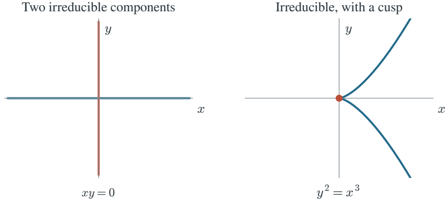
FIGURE 2. Reducible vs. irreducible algebraic sets in \mathbb{A}^2 . Left : V(xy) = V(x) \cup V(y) is the union of the two coordinate axes; I = (xy) , which is not prime, and \sqrt{I} = (x) \cap (y) records the two components. Right : the cuspidal cubic V(y^2 - x^3) is irreducible; its ideal (y^2 - x^3) is prime. A singular point (the cusp at the origin) does not prevent irreducibility.
