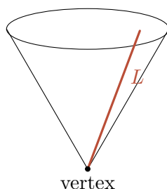
FIGURE 4. The quadric cone Q = V(xy - z^2) , the simplest singular surface. The ruling L = V(x, z) \subset Q is a prime Weil divisor that is not Cartier at the vertex: no single equation cuts it out there. Its double is: the function x vanishes on Q exactly along L , to order two, so \operatorname{div}(x) = 2L . Proposition 8.2 says smoothness rules out exactly this behaviour.
