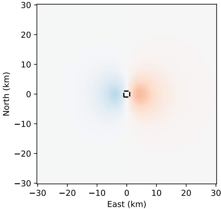
Sill: strike=0, dip=5, L=W=2km, op=10m, dc=8km
