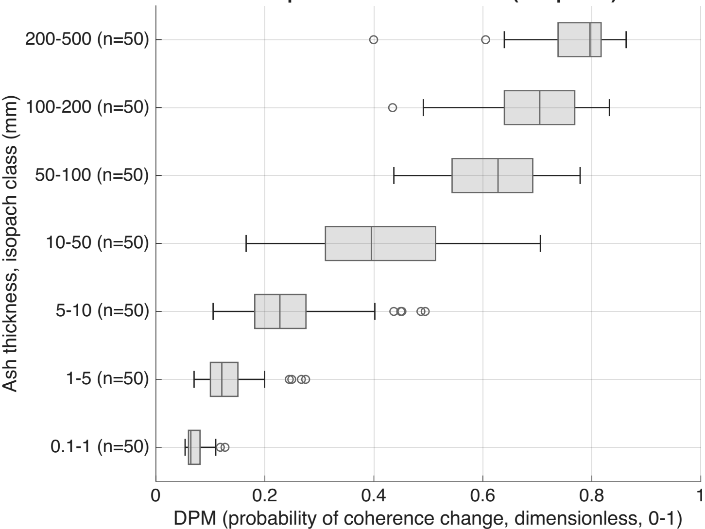
DPM per ash-thickness class (350 pixels)
