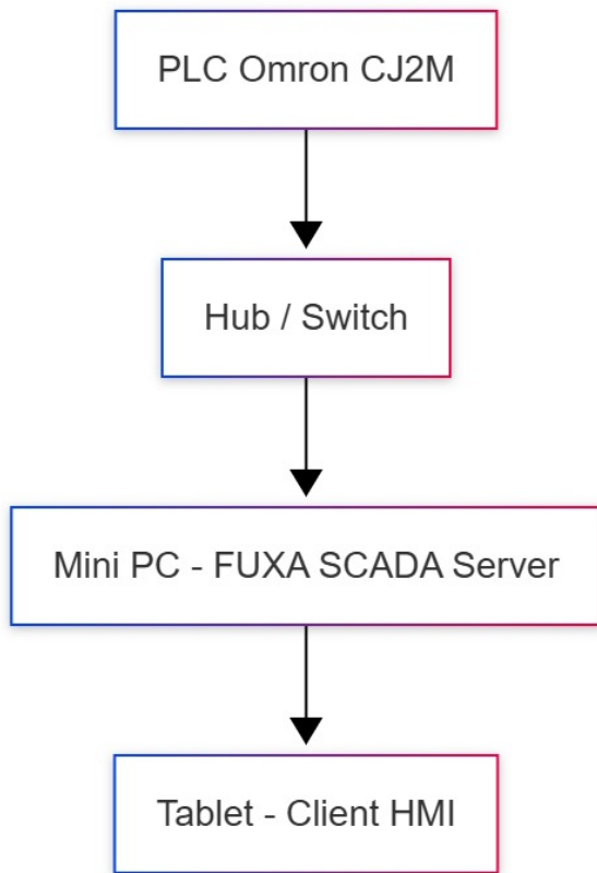
Figure 3: System topology of the FUXA HMI with the FINS connector
