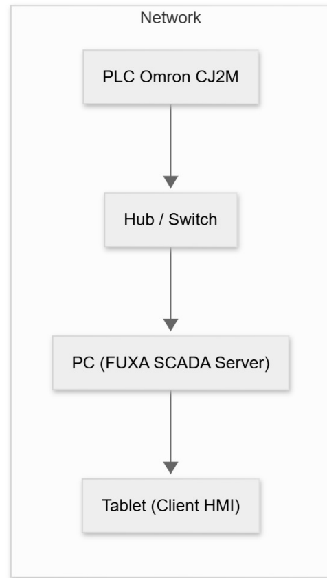
Figure 2: Architecture of the developed HMI-PLC communication system
