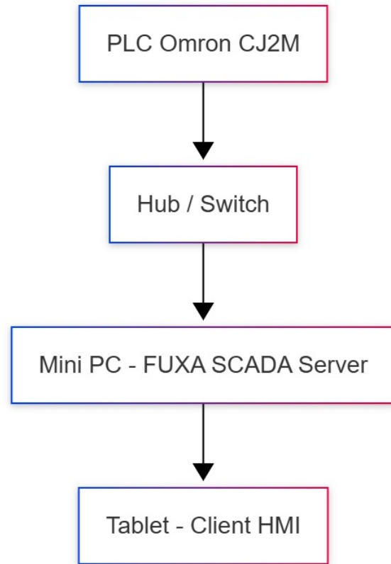
Figure 3: System topology of the FUXA HMI with the FINS connector
