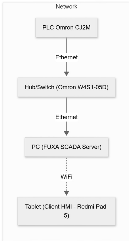
Fig. 3. System topology of the FUXA HMI with the FINS connector
