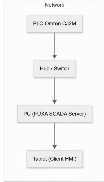
Fig. 2. Architecture of the developed HMI-PLC communication system
