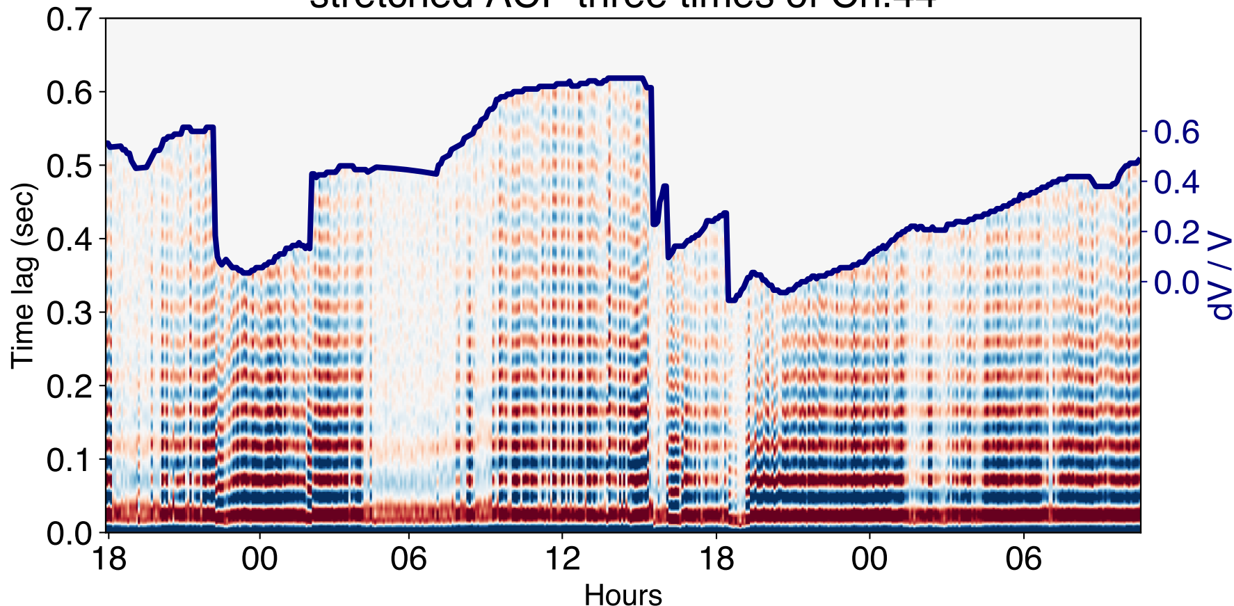
stretched ACF three times of Ch.44
