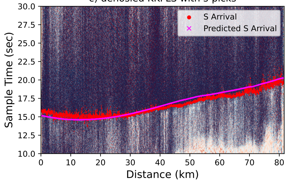
c) denoised KKFLS with s-picks
