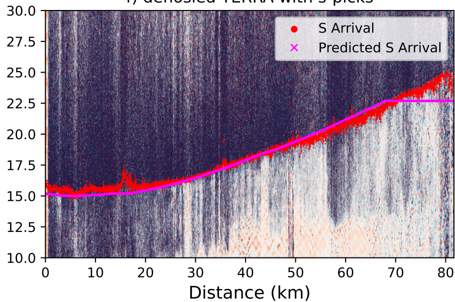
f) denoised TERRA with s-picks
