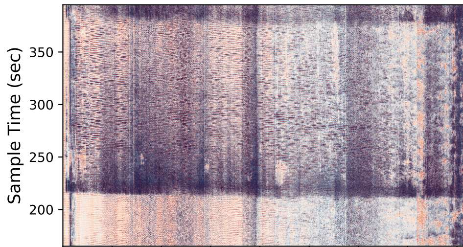
a) denosied KKFLS
