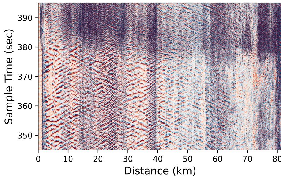
c) denosied KKFLS: S-wave
