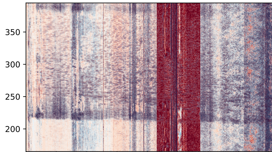
d) denosied TERRA
