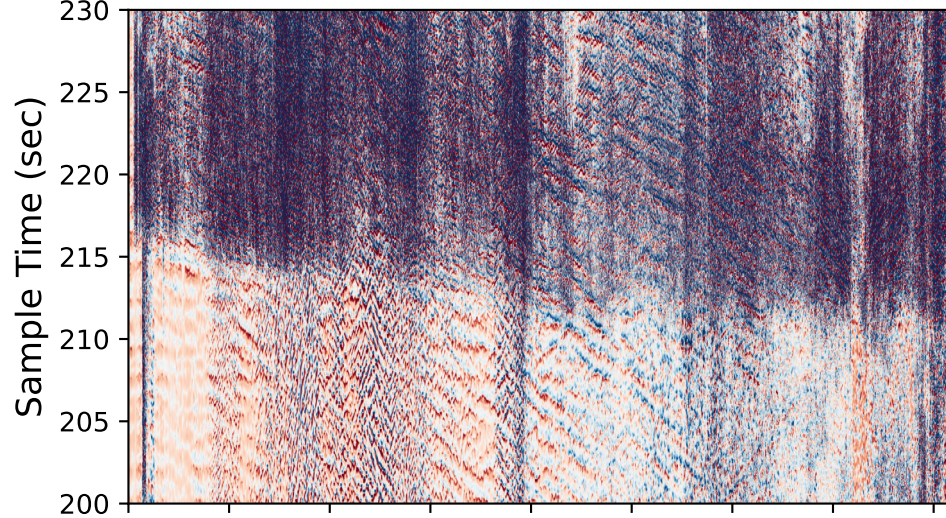
c) denosied KKFLS: S-wave
