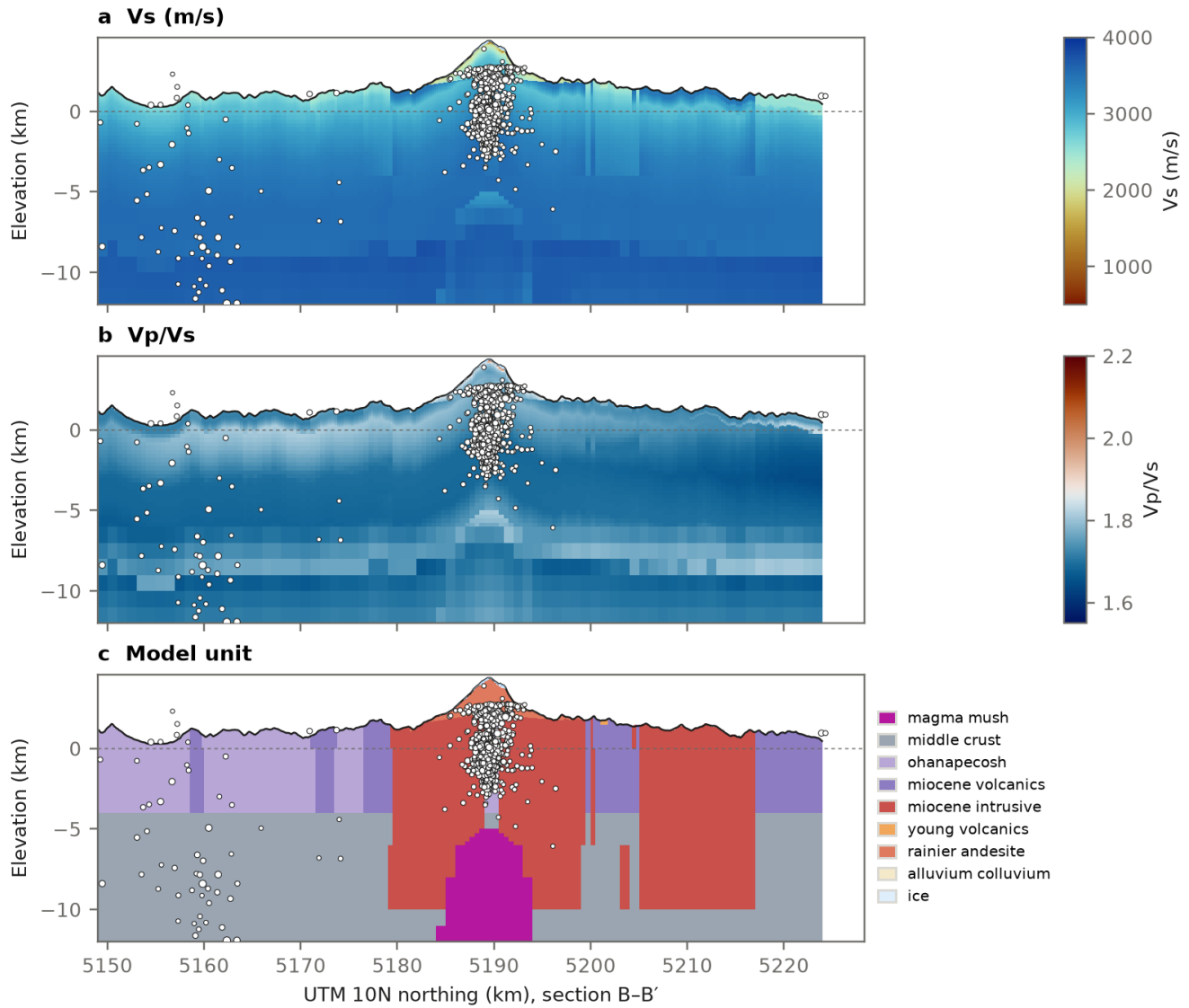
Figure 14. Fused model along B-B' (south-north through the summit): (a) Vs, (b) Vp/Vs, (c) model units. The step in Vp/Vs at 9.9 km below the ground (the base of the Cascadia model used, CVM_MAX_DEPTH in rainier3d.fusion.regional ) marks the change from the Cascadia model to CRESCENT with Brocher's Vp.
