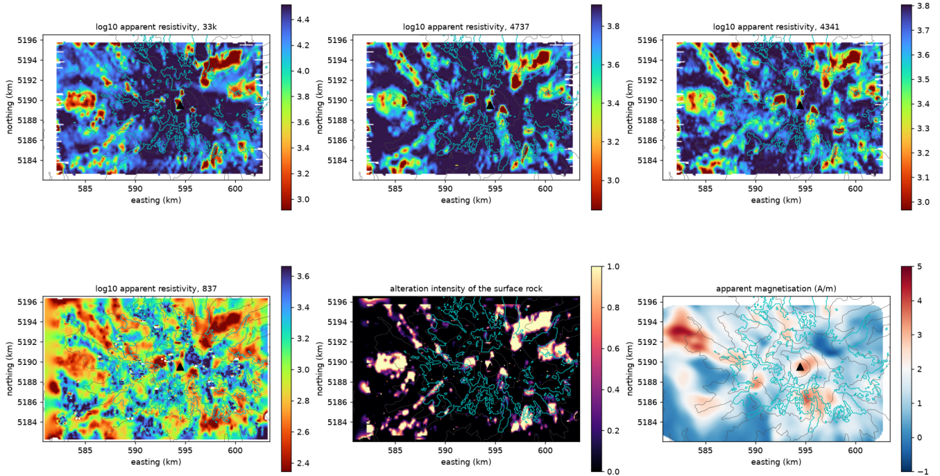
Figure 6. Apparent resistivity at the four EM frequencies, alteration intensity of the surface rock and terrain-correlated apparent magnetisation (S22). Contours: elevation every 500 m; cyan: glaciers thicker than 10 m; triangle: summit.
