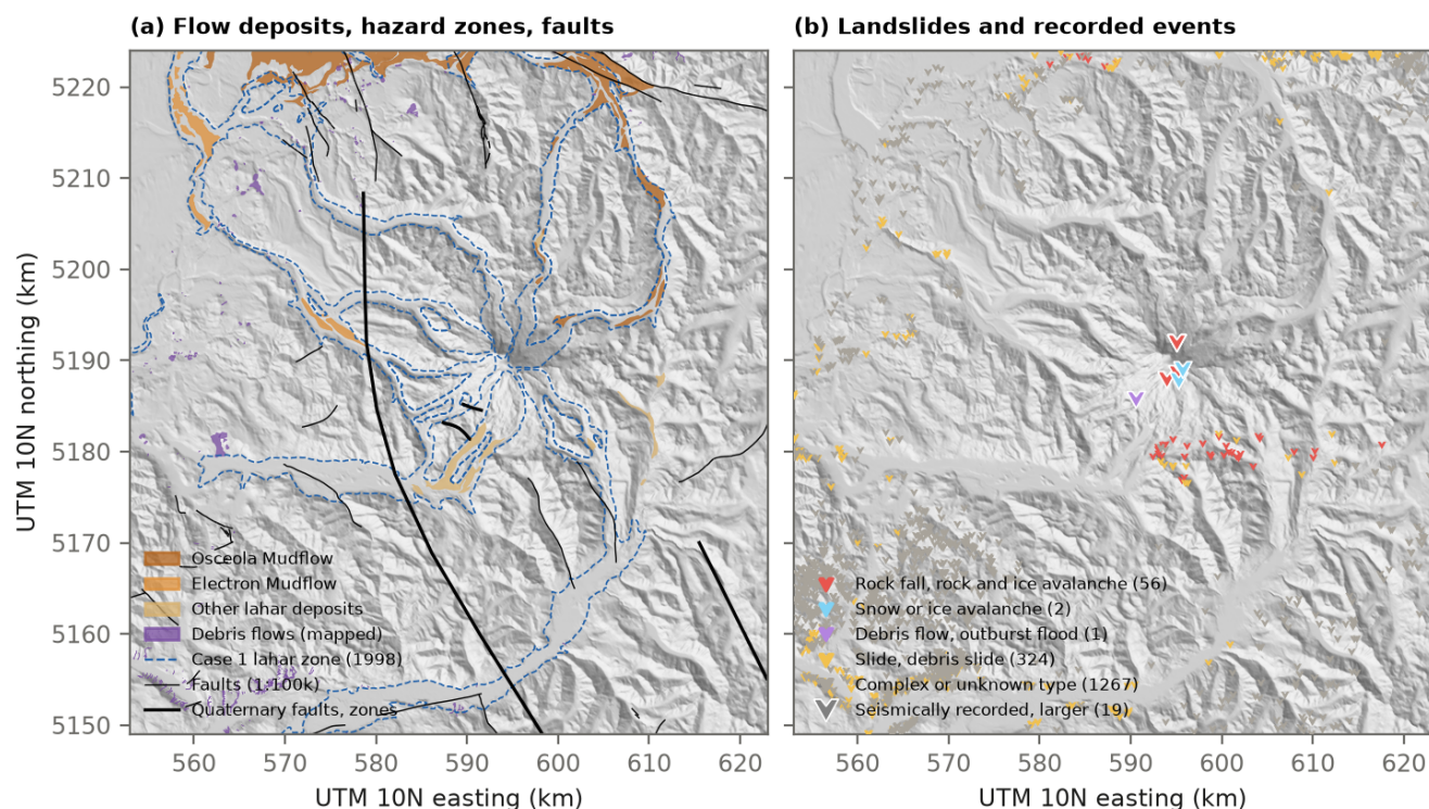
Figure 21. Mass movements and faults. (a) Lahar deposits and mapped debris flows, the case 1 lahar inundation zone of 1998 (dashed), and faults of the 1:100,000 map (thin) and of the Quaternary fault layer (thick). (b) Events by class, drawn as downward chevrons as in the viewer: landslides at their crown (small) and seismically recorded events (large, white rim).
