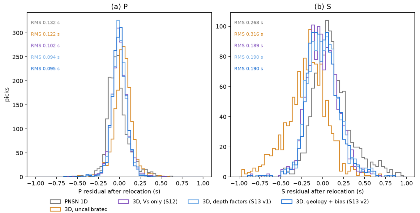
Figure 10. P (a) and S (b) residuals after relocating all events in each model; the RMS of each model is printed in its colour.
