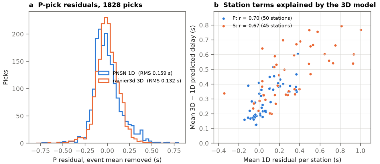
Figure 15. At the ComCat hypocentres: (a) distribution of P residuals after removing each event's mean, for the PNSN 1D model and the fused model; (b) mean 3D - 1D predicted delay against mean 1D residual for each station with at least five picks.
