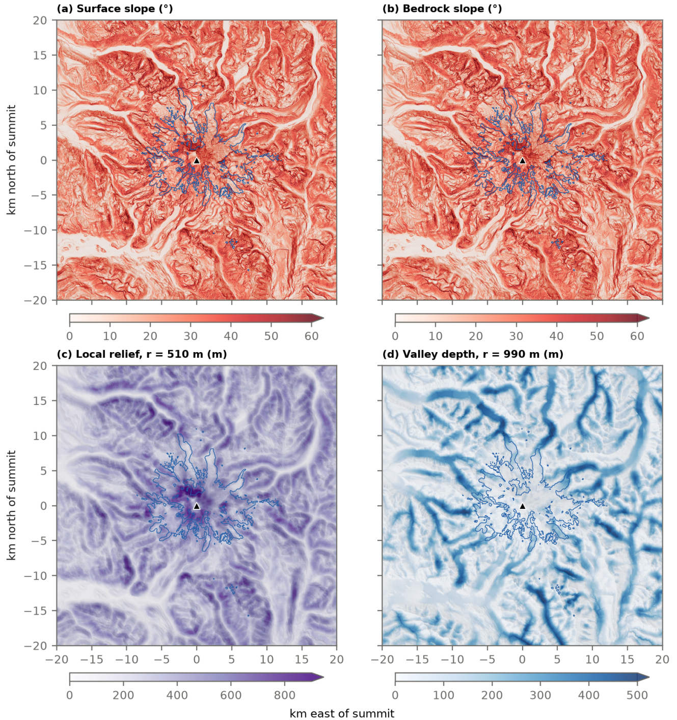
Figure 7. Terrain geometry over 40 \times 40 km centred on the summit (triangle), on the 30 m grid (S30): (a) surface slope, \arctan |\nabla z| from central differences between adjacent cells (60 m baseline), the slope of the ice surface on glaciers; (b) bedrock slope, the same operator on the 3DEP elevation minus the IceBoost v2 thickness (bilinear from 100 m), identical to (a) off the ice; (c) local relief, maximum minus minimum elevation within a disk of radius 510 m; (d) valley depth, the grey-scale closing of the elevation with a disk of radius 990 m minus the elevation. Filters mirror-reflect at the grid edges. The blue line outlines ice thicker than 10 m. The 35–49 m effective resolution of the source smooths cliffs, the bedrock slope inherits the errors of the ice thickness, and the radii are adjustable.
