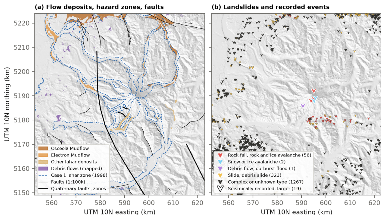
Figure 24. Mass movements and faults. (a) Lahar deposits and mapped debris flows, the case 1 lahar inundation zone of 1998 (dashed), and faults of the 1:100,000 map (thin) and of the Quaternary fault layer (thick). (b) Events by class, drawn as downward chevrons as in the viewer: landslides at their crown (small) and seismically recorded events (large, white rim).
