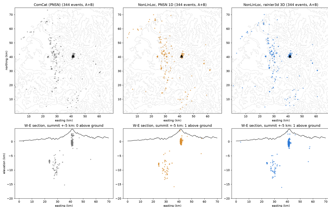
Figure 25. The 2023–2025 PNSN catalogue (magnitude \geq 1 ; the 344 events graded A or B in rainier3d) as located by ComCat, by NonLinLoc in the PNSN 1D model and by NonLinLoc in rainier3d. Top: epicentres over elevation contours. Bottom: west–east sections within 5 km of the summit, with the ground profile, and the number of events above the ground.
