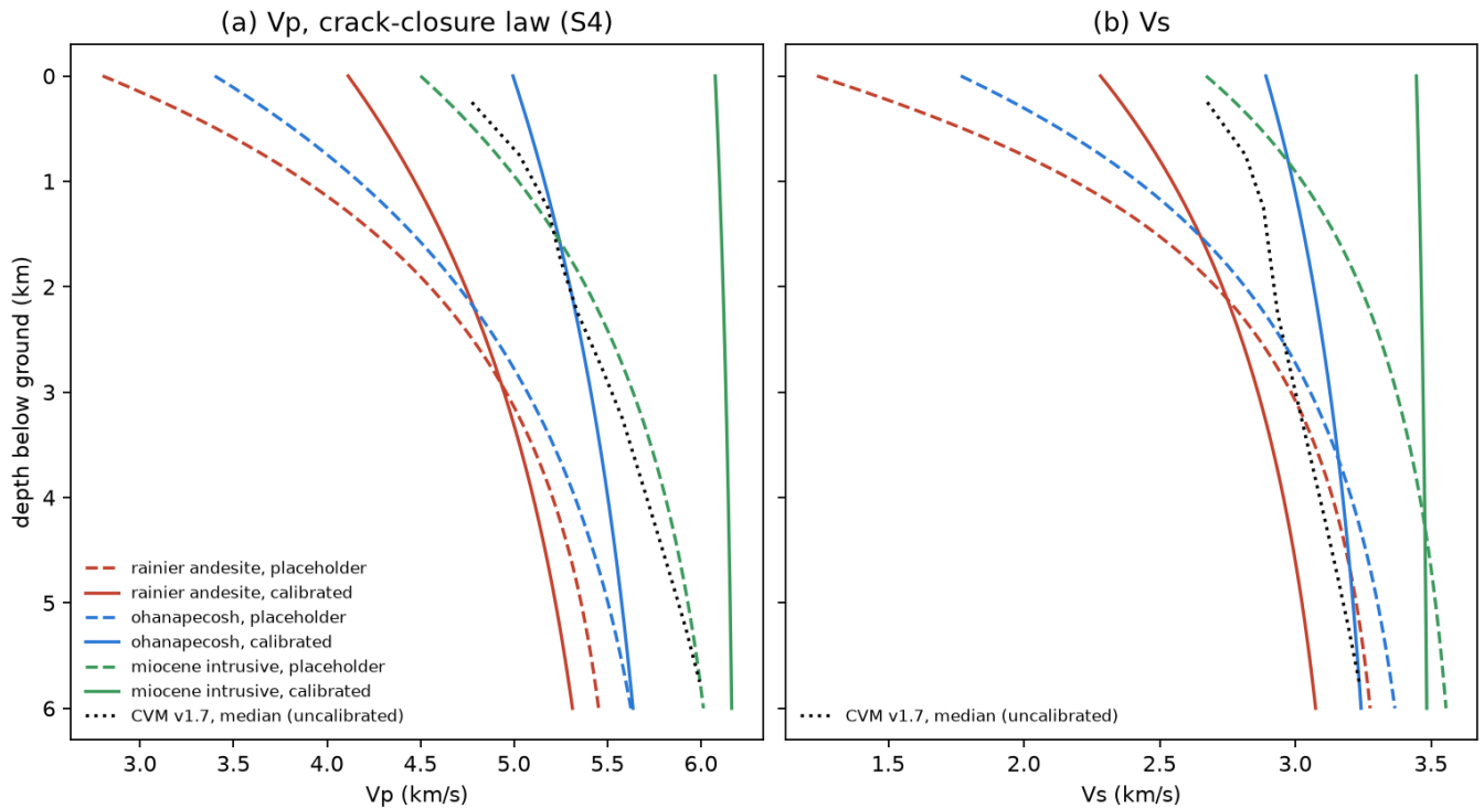
Figure 12. Crack-closure Vp (a) and Vs (b) against depth below ground for three rock units, with table (dashed) and calibrated (solid) parameters. Dotted: median of the Cascadia velocity model over the domain.
