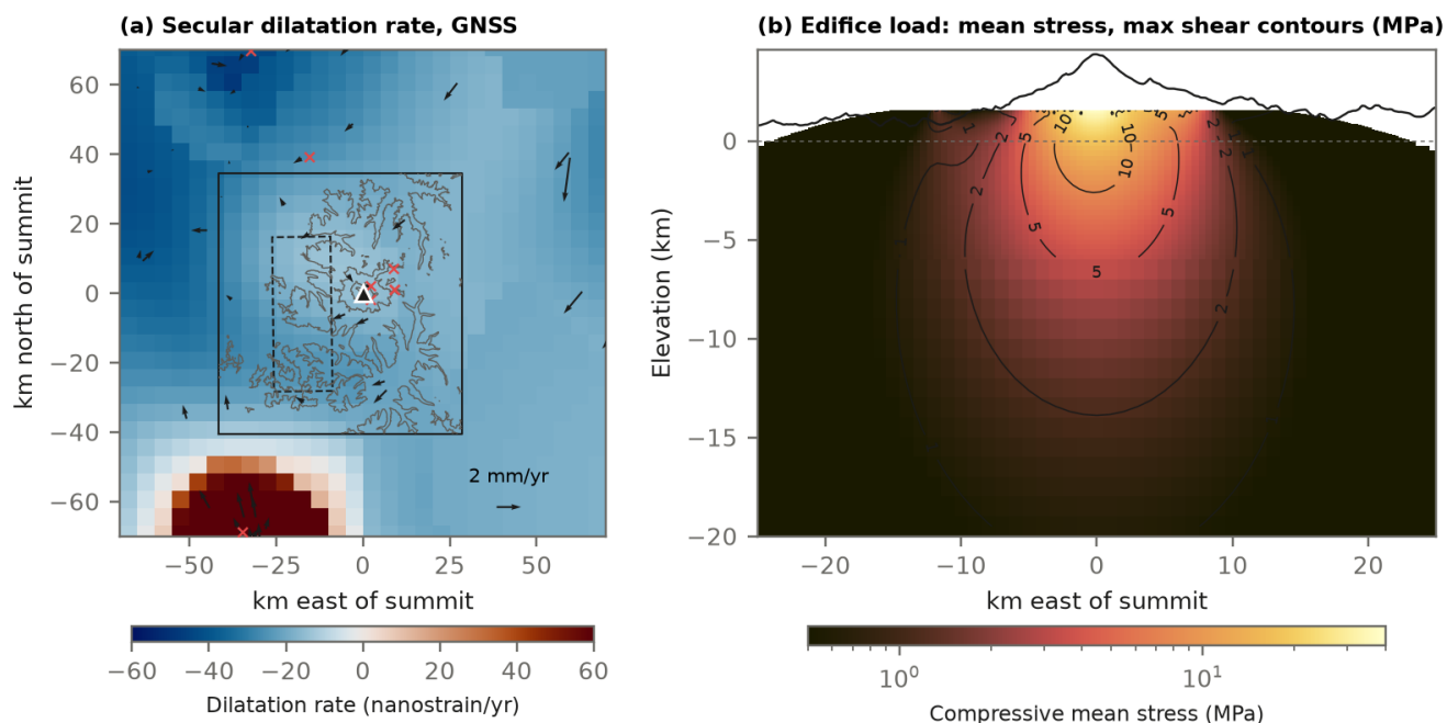
Figure 20. (a) Secular dilatation rate from the GNSS velocities, with the velocities of quality-controlled sites relative to the network median (arrows) and flagged sites (red crosses). The solid box is the model domain and the dashed polygon the WRSZ region. (b) Compressive mean stress from the edifice load along a west–east section through the summit, with contours of maximum shear (MPa).
