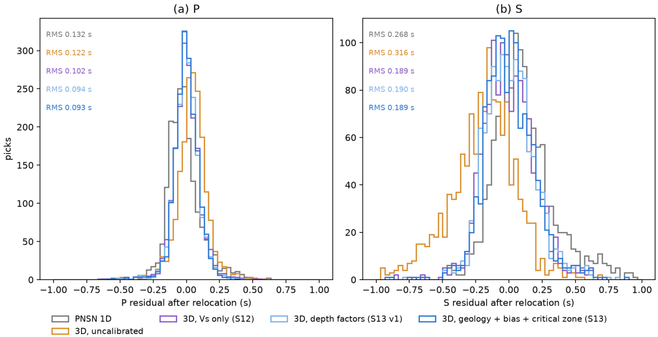
Figure 13. P (a) and S (b) residuals after relocating all events in each model; the RMS of each model is printed in its colour.
