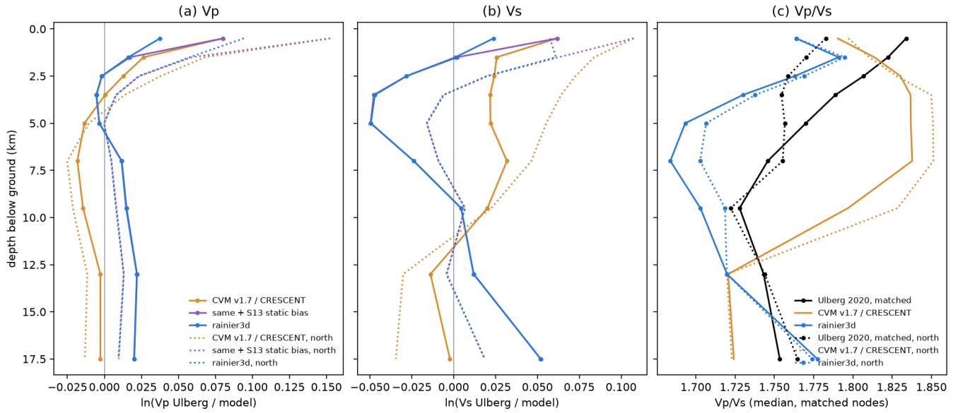
Figure 14. rainier3d and the regional models against the iMUSH tomography. (a, b) Mean \ln(V_{\text{iMUSH}}/V_{\text{model}}) against depth below ground, over the box (solid) and north of 46.75^\circ N (dotted). (c) Median Vp/Vs where the iMUSH P and S models are both resolved.
