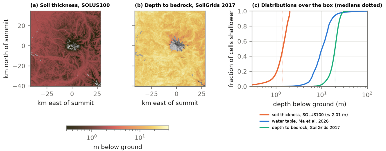
Figure 5. Depth to rock from two sources on one logarithmic scale: (a) SOLUS100 soil thickness (depth to a lithic contact, capped at 2.01 m); (b) SoilGrids250m 2017 depth to bedrock; (c) distributions over the box of the two depths and of the Ma et al. (2026) water-table depth, with medians dotted. Glacier cells are left empty. The order-of-magnitude gap between the two depths contains the water table.
