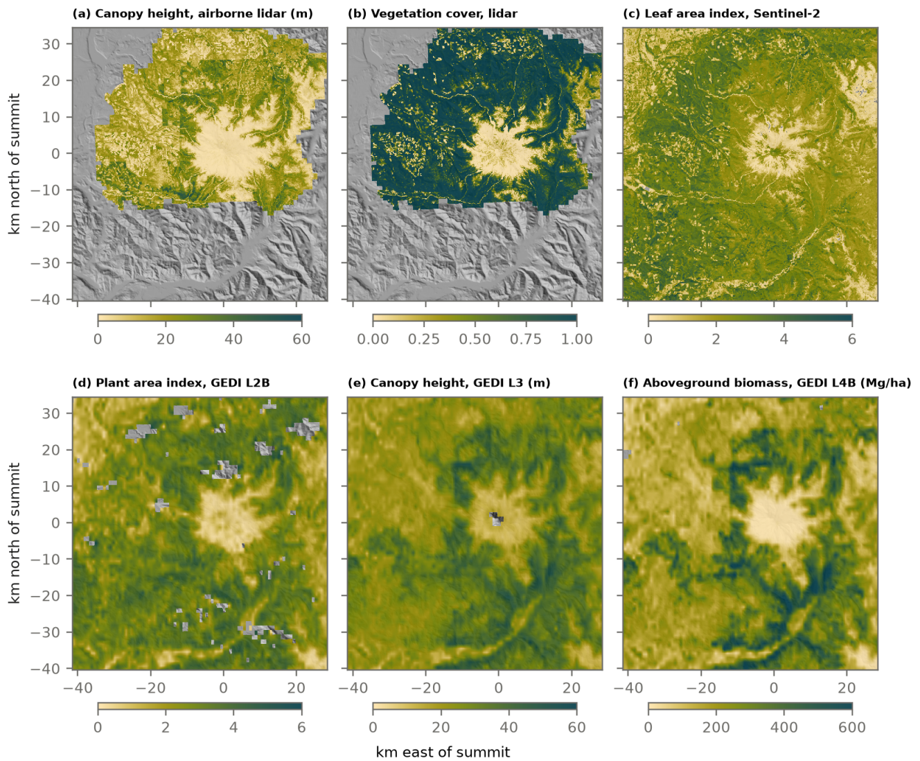
Figure 6. Vegetation layers on the model grid, over a hillshade: (a) lidar canopy height and (b) vegetation cover, (c) Sentinel-2 leaf area index, (d) GEDI plant area index, (e) GEDI canopy height, (f) GEDI aboveground biomass. Straight edges in (a) and (b) are lidar tile boundaries.
