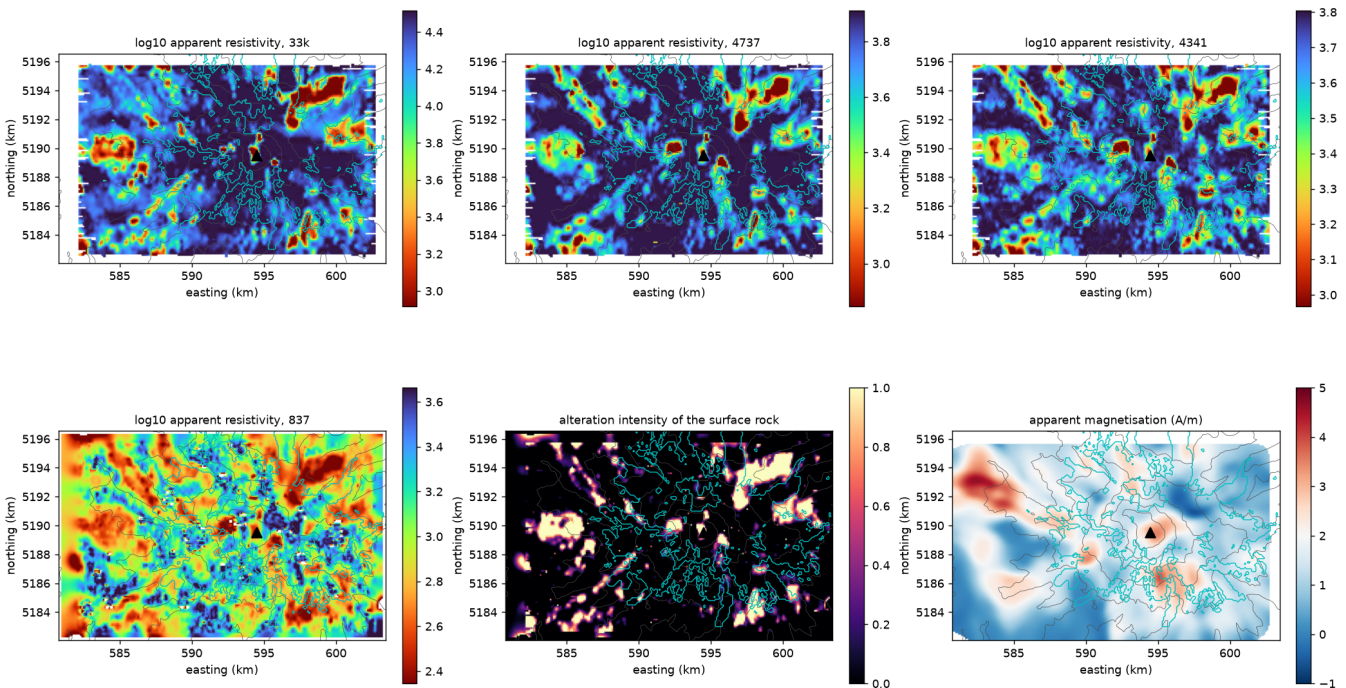
Figure 9. Apparent resistivity at the four EM frequencies, alteration intensity of the surface rock and terrain-correlated apparent magnetisation (S22). Contours: elevation every 500 m; cyan: glaciers thicker than 10 m; triangle: summit.
