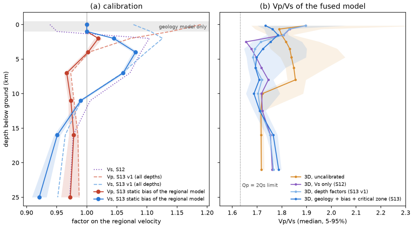
Figure 11. (a) Static correction of the regional Vp and Vs (solid, \pm 1 standard deviation). The dashed and dotted lines are the two alternative parameterisations of Table 18. The grey band is the geology-only zone. (b) Median and 5–95% range of Vp/Vs of the fused model against depth below ground.
