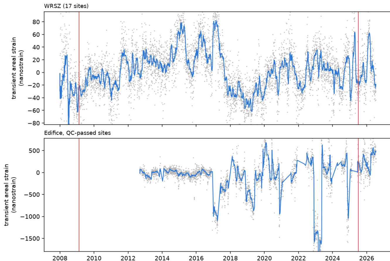
Figure 19. Daily areal strain of the stations around the WRSZ and the edifice, from trajectory residuals (grey), with 30-day medians (blue). Red lines mark the 2009 and 2025 summit swarms.
