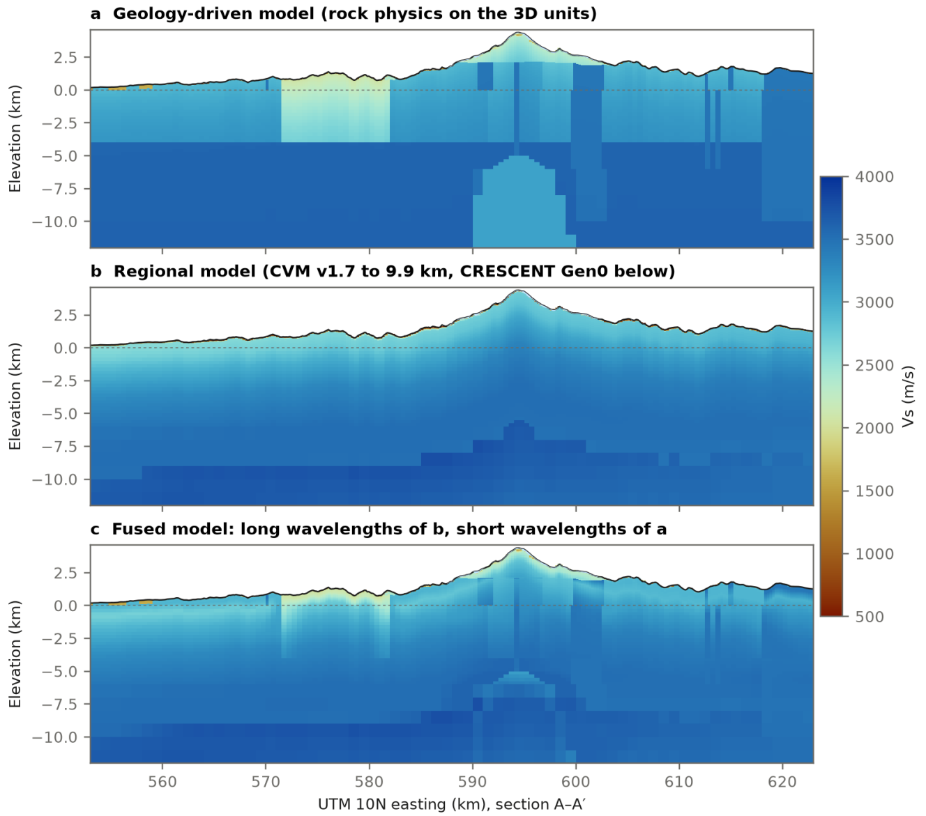
Figure 10. Vs along section A–A' (west–east through the summit): (a) geology model, (b) regional model, (c) fused model. The fused model keeps the regional long wavelengths and the geological contrasts: the Puget Group sedimentary block near 572–582 km, the Tatoosh and White River plutons, and the slow edifice.
