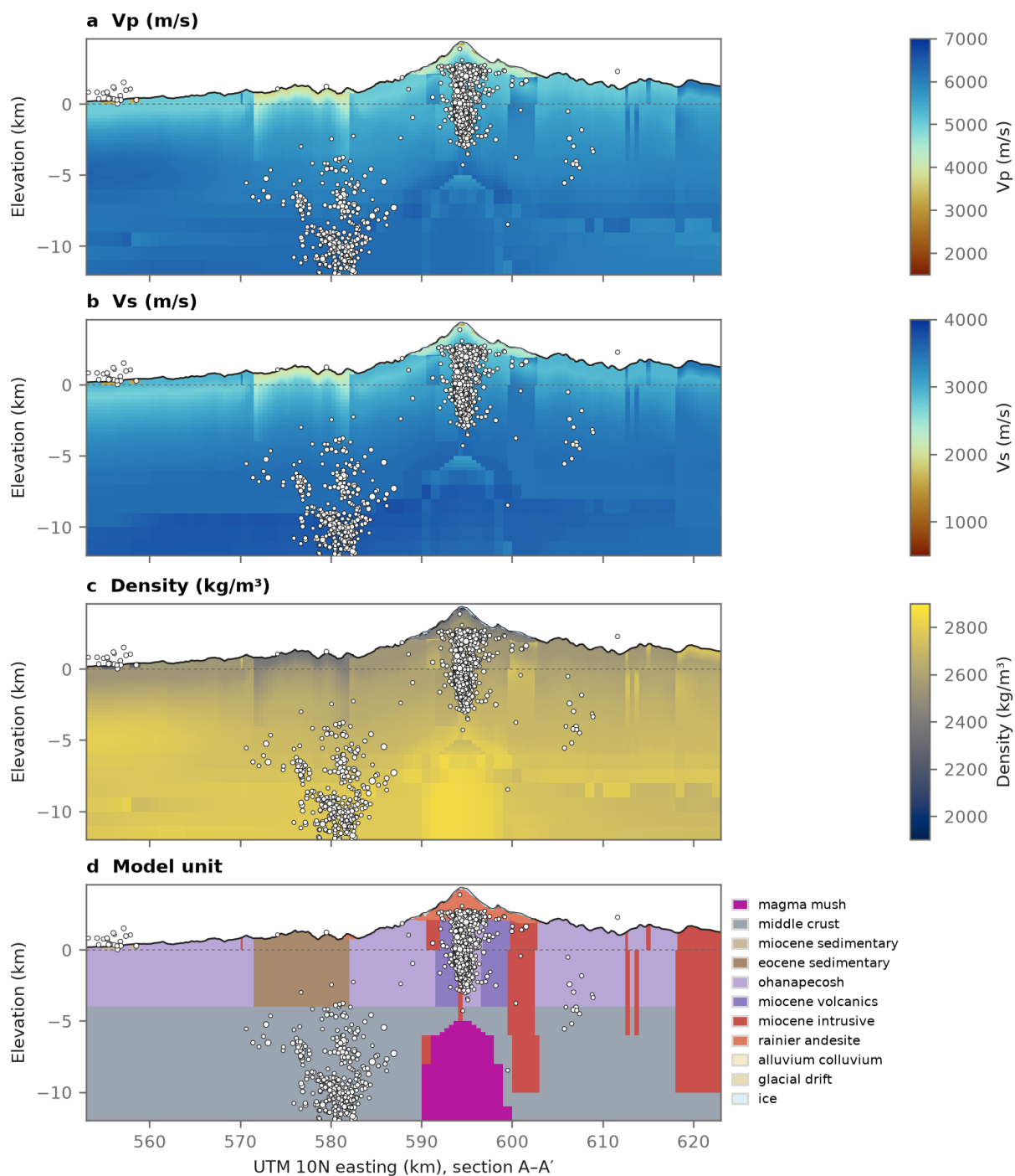
Figure 16. Fused model along A–A' (west–east through the summit): (a) Vp, (b) Vs, (c) density, (d) model units. Light blue at the surface is glacier ice. White dots are PNSN earthquakes within 2 km of the section. The dashed line is sea level.
