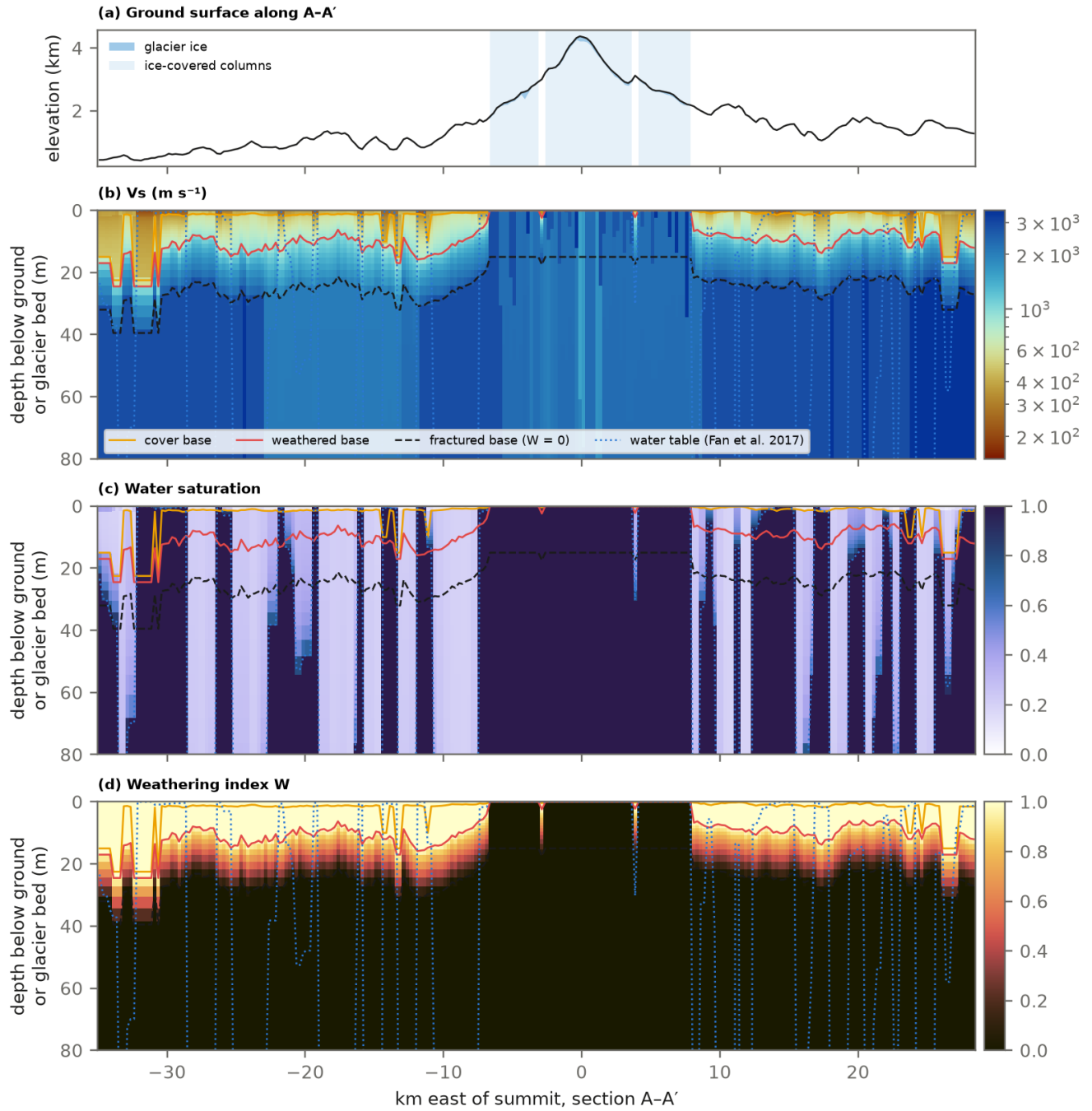
Figure 8. The critical zone along A-A' (west-east through the summit; the /cz node of model.zarr , S4). (a) Ground surface, with glacier ice and the ice-covered columns shaded. (b) Vs, (c) water saturation and (d) weathering index W against depth below the ground or the glacier bed, with the bases of the Quaternary cover, the weathered layer and the fractured zone, and the water table of Fan et al. (2017). Under ice the columns start in fractured rock saturated from the bed ( W = 0 ). Depths below 80 m are not shown; Vs joins the L1 cells at 150 m.
