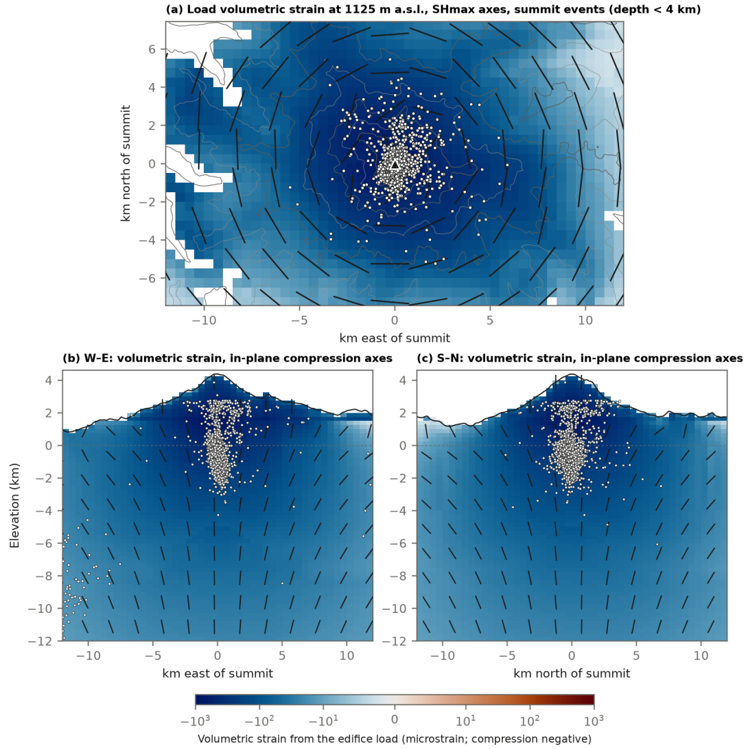
Figure 22. Static strain of the edifice load. (a) Volumetric strain at 1125 m above sea level, with the direction of the most compressive horizontal stress (SHmax, bars) and the summit earthquakes shallower than 4 km (dots). (b, c) West–east and south–north sections through the summit, with the in-plane axis of maximum compression; inside the cone, the confined overburden makes it vertical.
