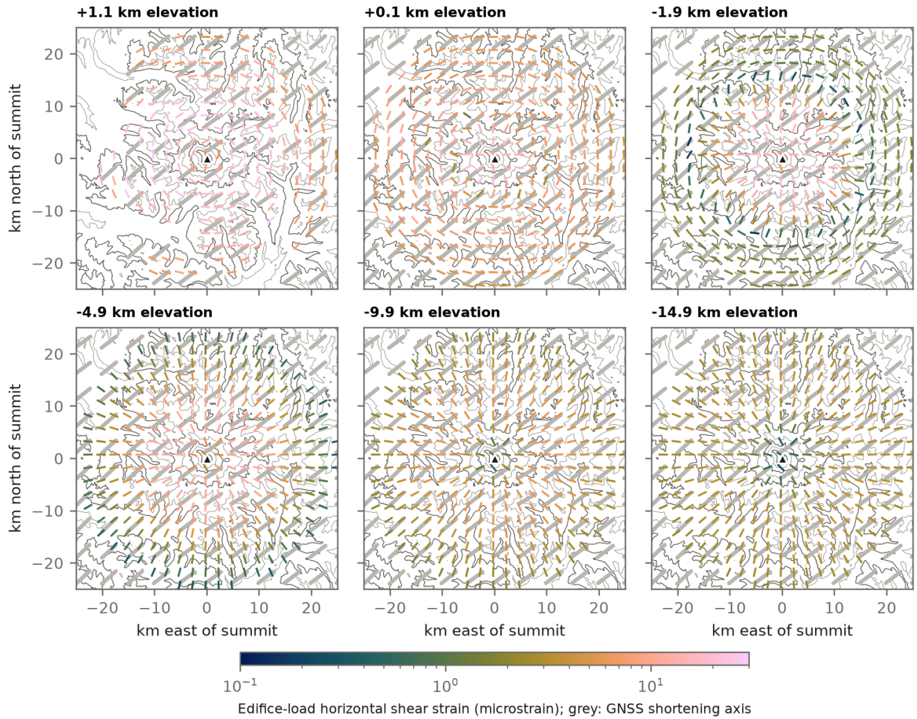
Figure 23. Axes of maximum horizontal shortening at six elevations: GNSS (grey, the same at every depth) and SHmax of the edifice load (coloured by its horizontal shear strain).
