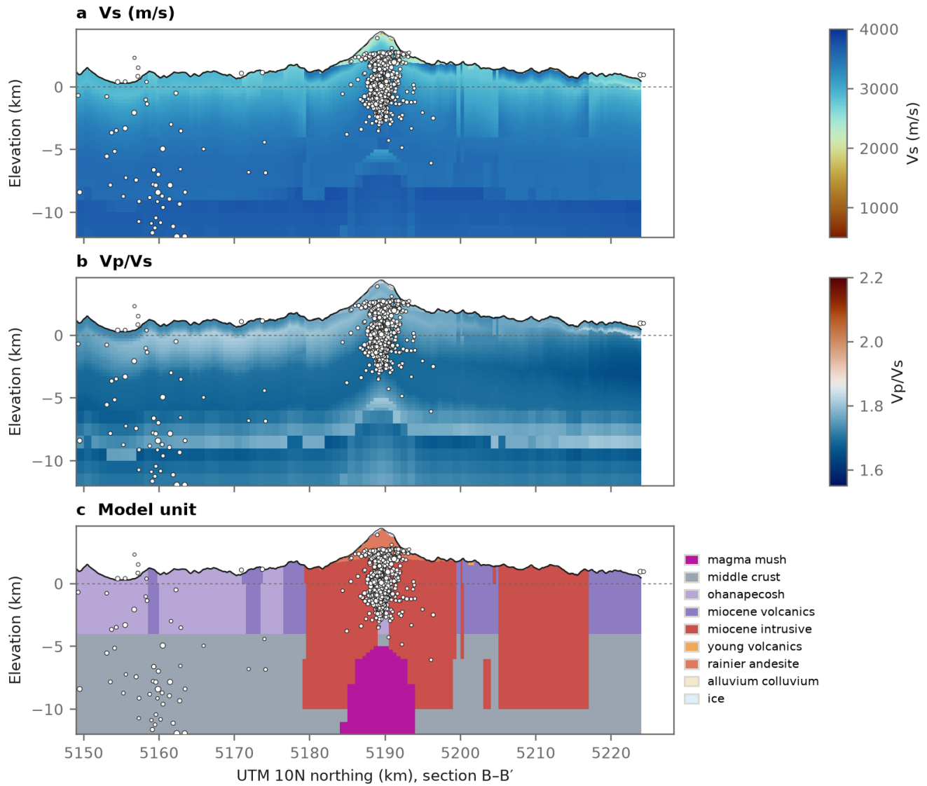
Figure 17. Fused model along B-B' (south-north through the summit): (a) Vs, (b) Vp/Vs, (c) model units. The step in Vp/Vs at 9.9 km below the ground (the base of the Cascadia model used, CVM_MAX_DEPTH in rainier3d.fusion.regional ) marks the change from the Cascadia model to CRESCENT with Brocher's Vp.
