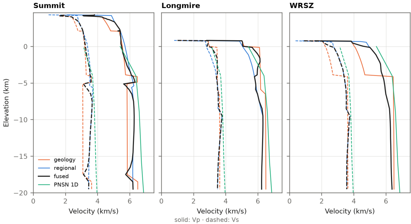
Figure 18. Vertical profiles of Vp (solid) and Vs (dashed) at the summit, at Longmire and in the WRSZ, for the geology, regional and fused models and the PNSN 1D model.
