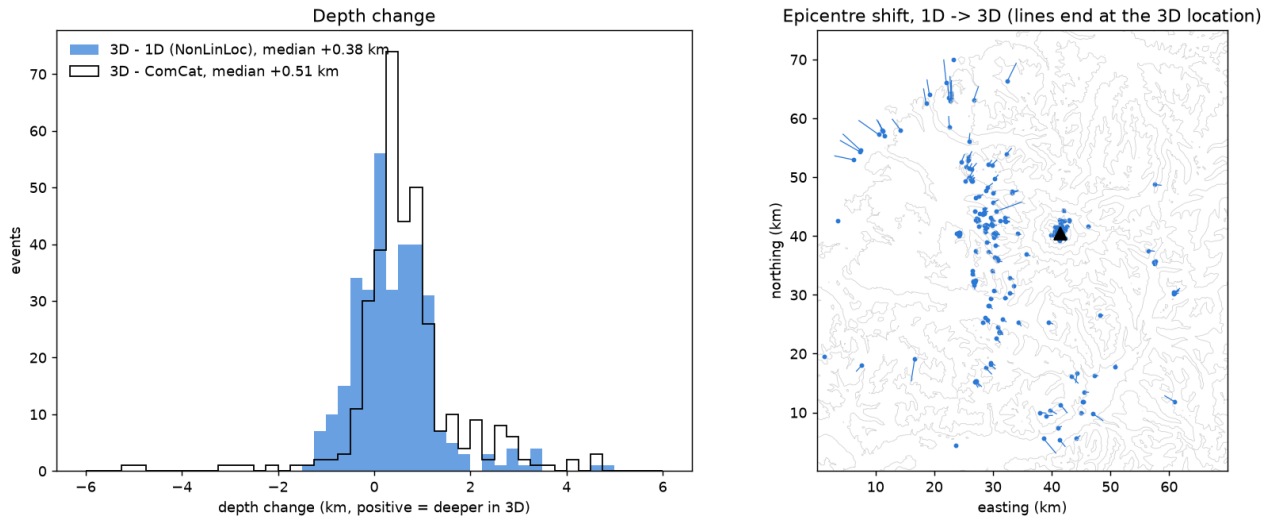
Figure 26. (a) Depth change of each event between rainier3d and the 1D model (filled) and between rainier3d and ComCat (outline). (b) Epicentre shifts from the 1D to the 3D location.
