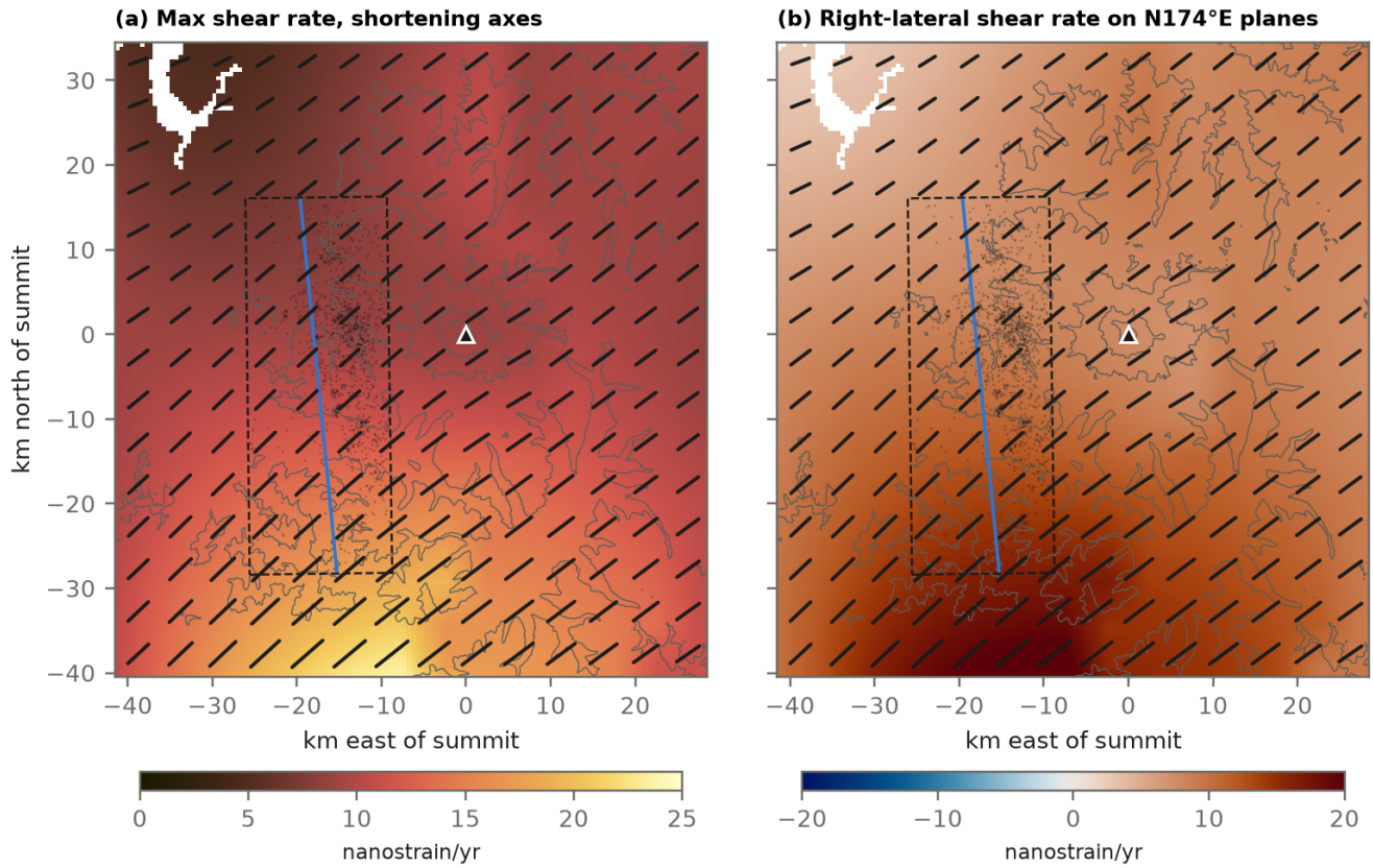
Figure 21. Tectonic strain rate from GNSS, the same at every depth under the stated assumptions: (a) maximum horizontal shear strain rate with the axes of maximum shortening (bars, length scaled with the shear rate); (b) right-lateral shear strain rate on vertical planes parallel to the WRSZ. The dashed polygon is the WRSZ region, grey dots its epicentres, and the blue line the strike fitted to them.
