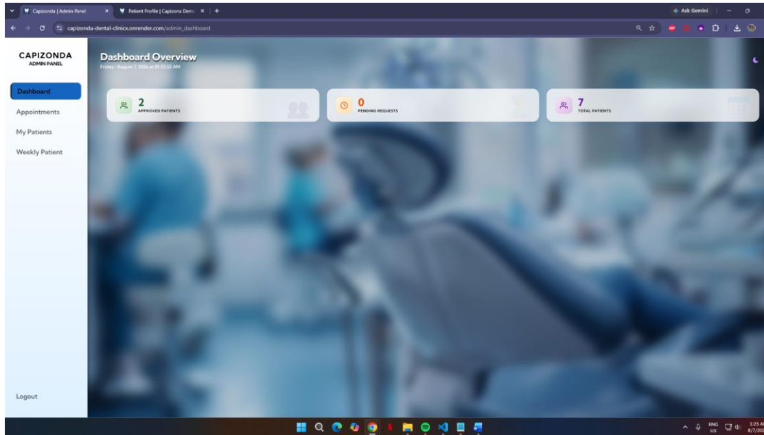
Figure 4.6 Admin Dashboard
