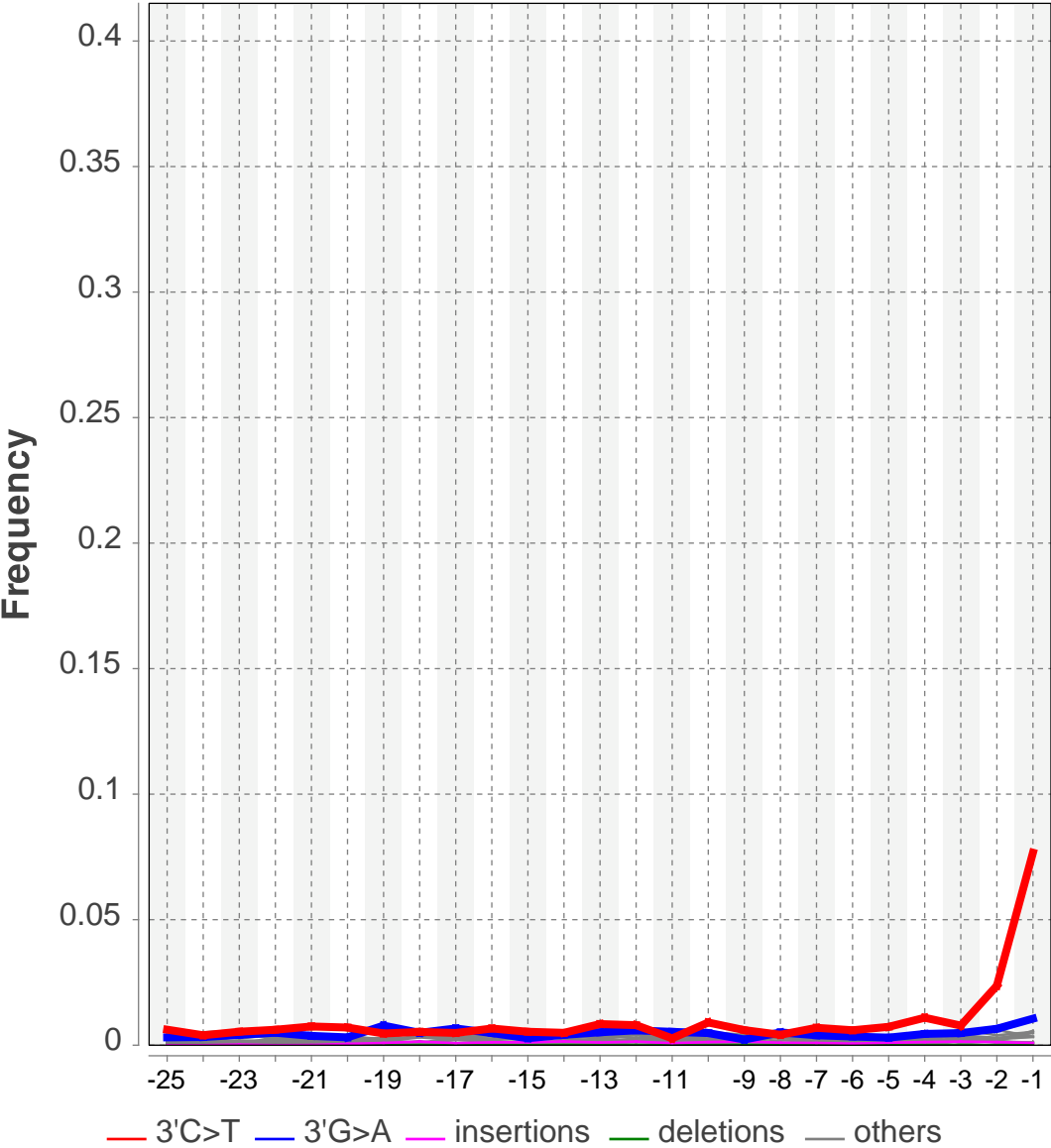
3' end
