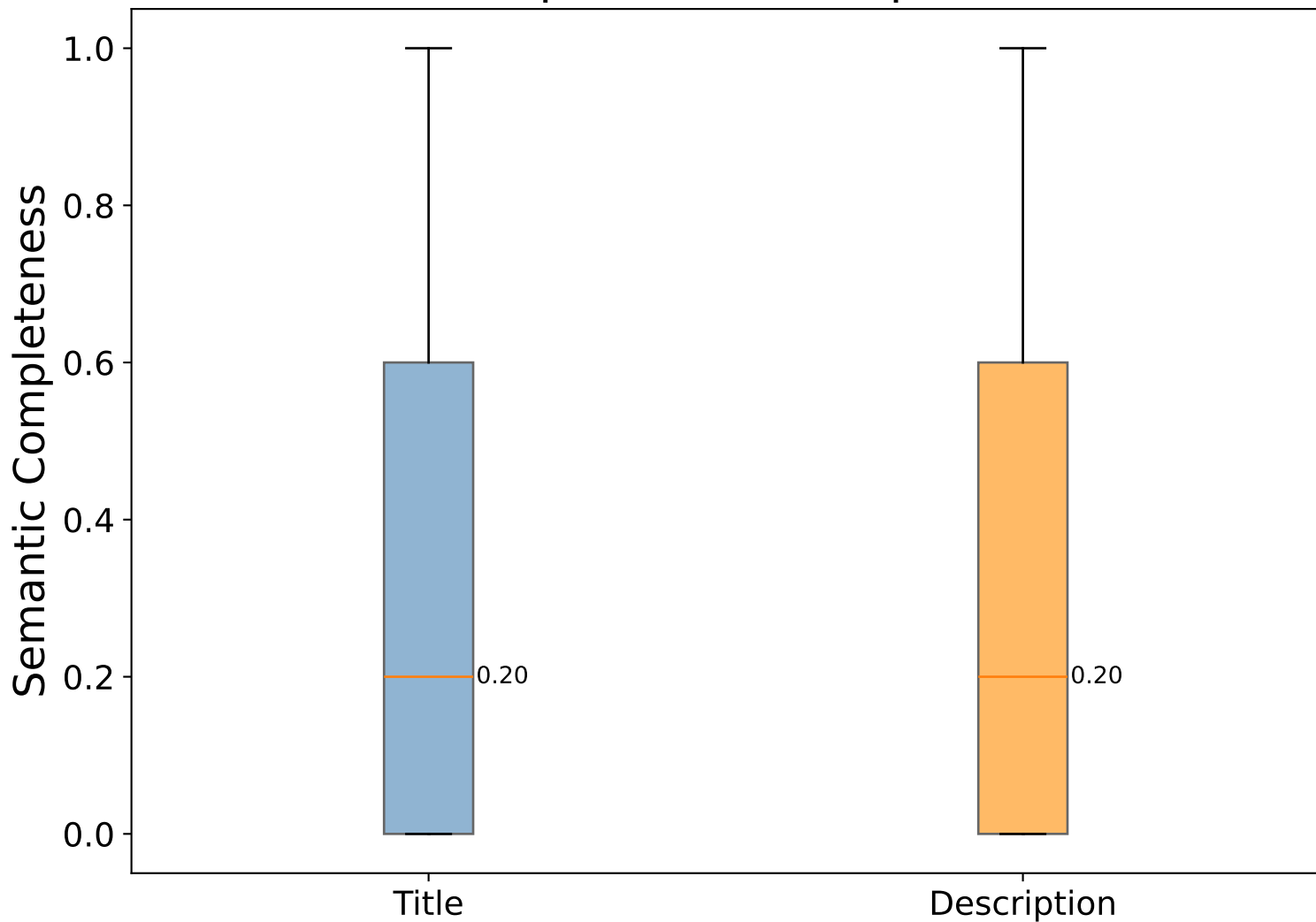
Semantic Completeness Comparison ( \tau=0.7 )
