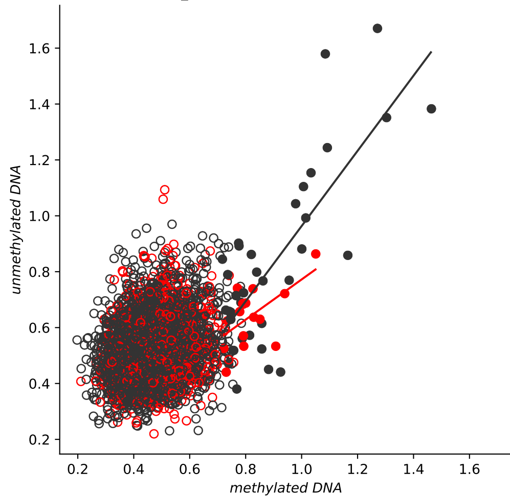
ZNF891_FL 6 enrichment, normalized by input
