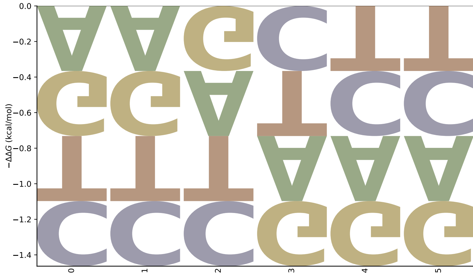
ZNF891_FL unmethyated bindingmode 3
