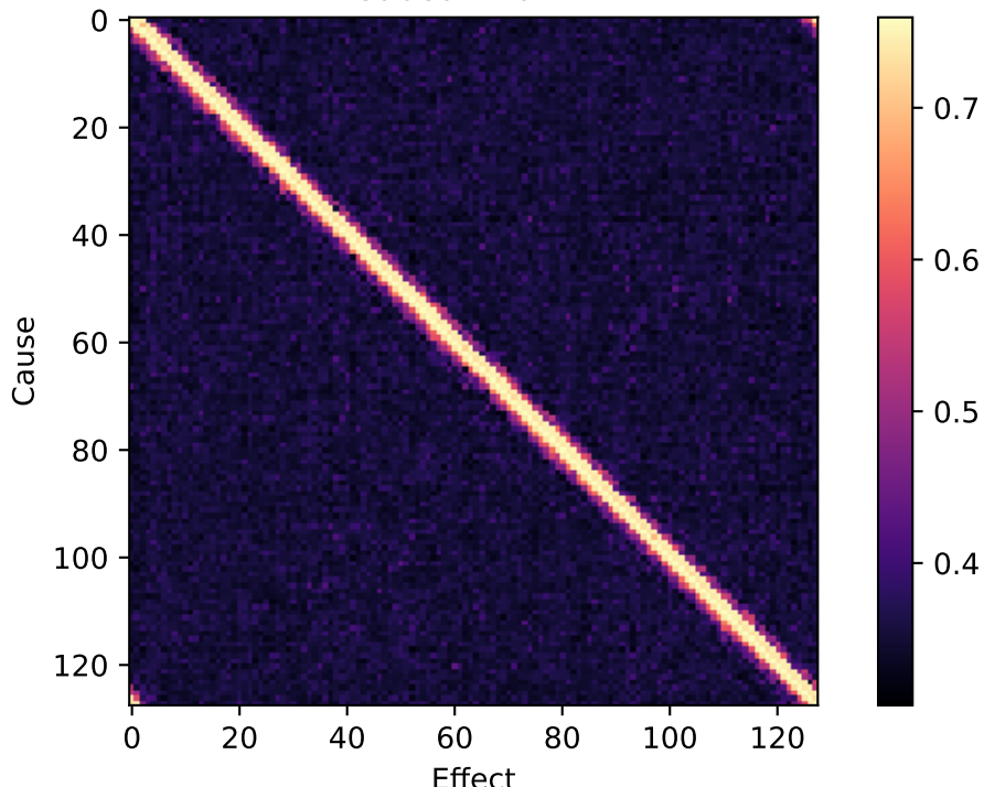
Causal matrix
