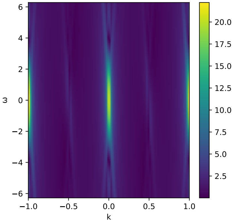
S(k, \omega) for g=2 , h=0.1 , J=1
