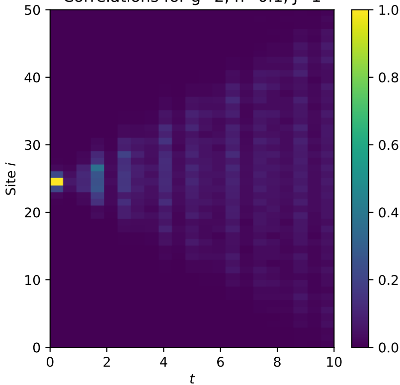
Correlations for g=2 , h=0.1 , J=1
